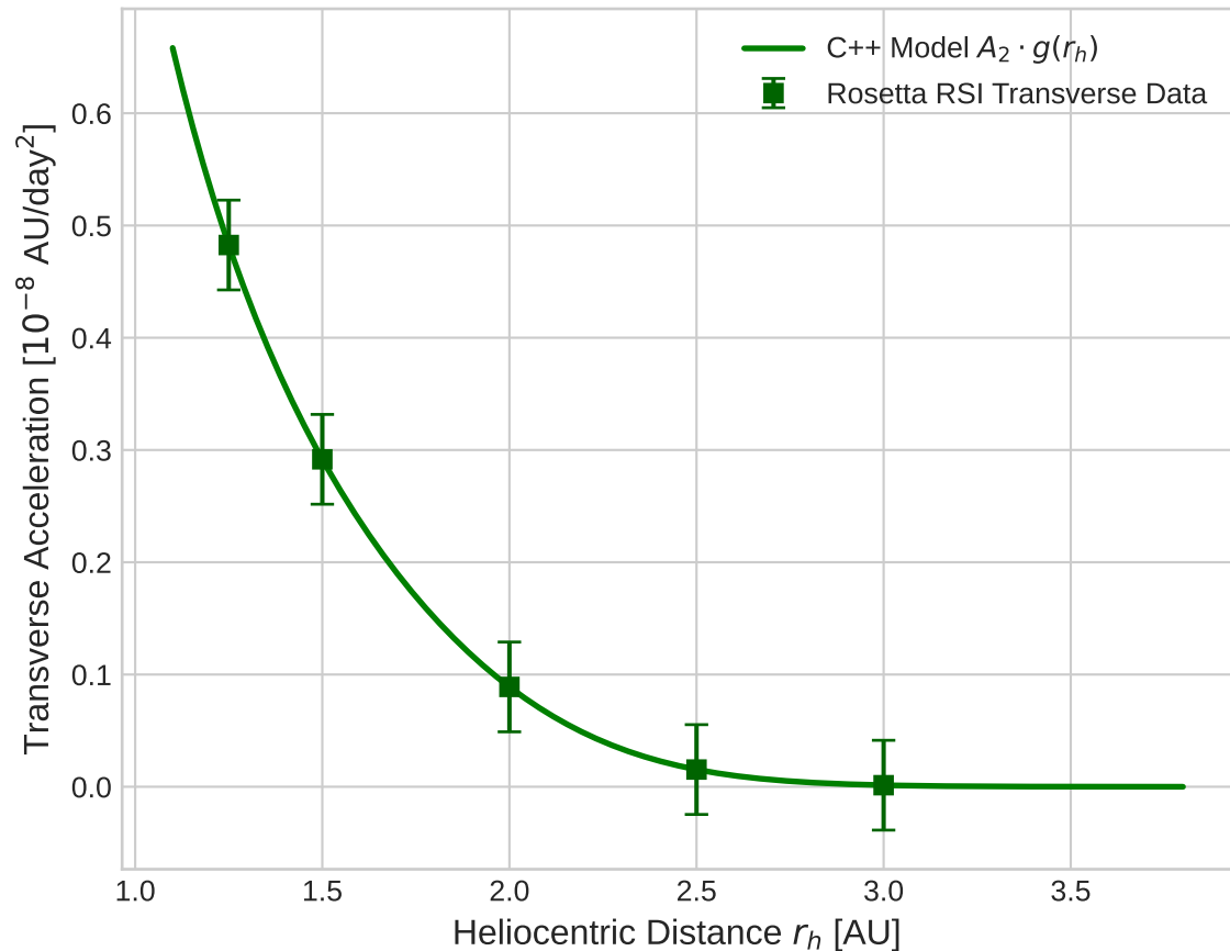
Transverse Non-Gravitational Acceleration Comparison
