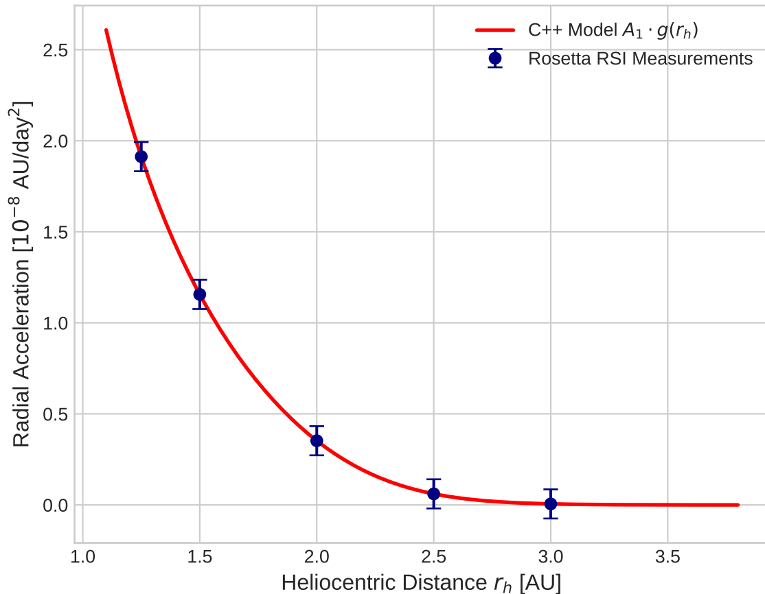
Radial Non-Gravitational Acceleration Comparison
