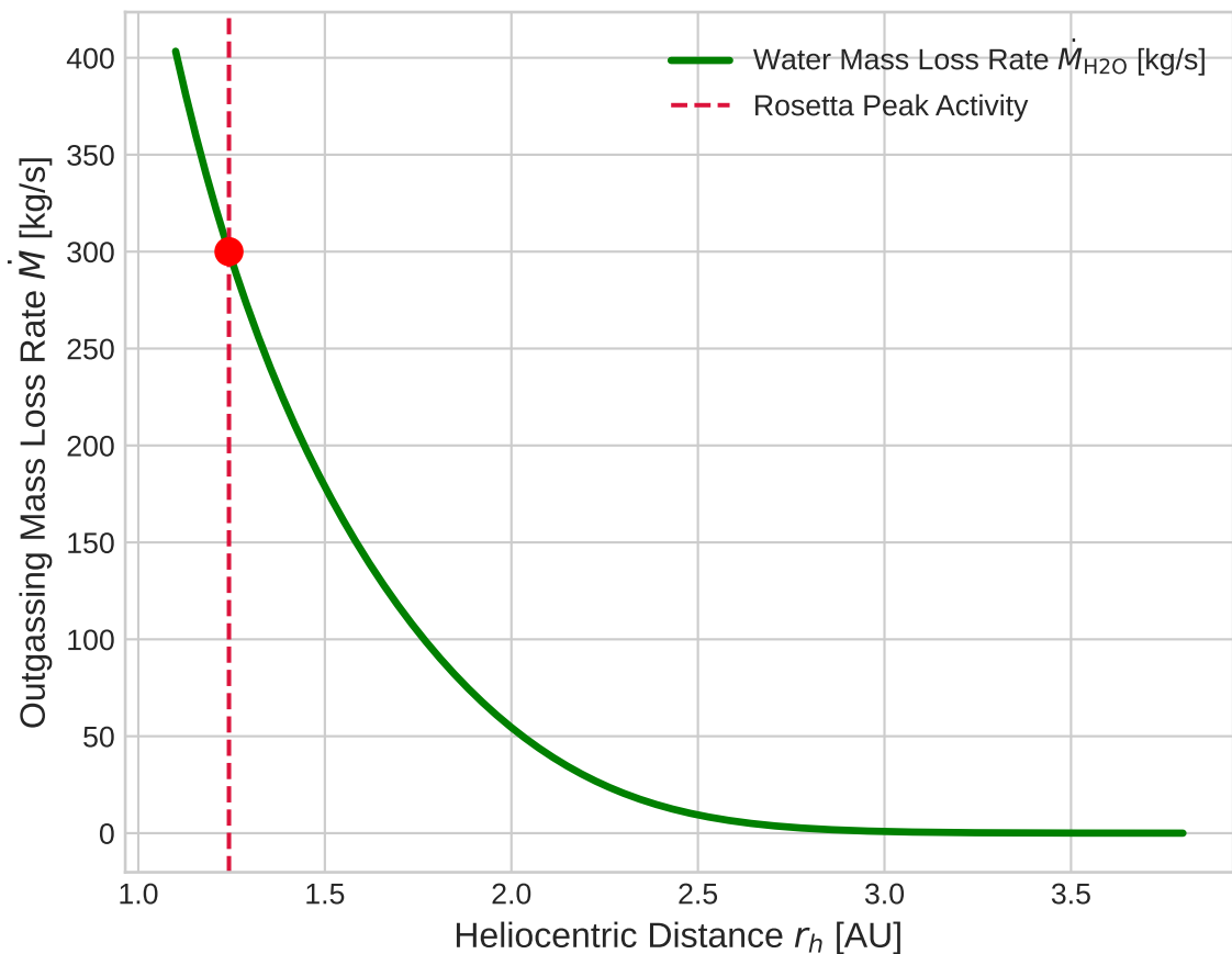
Sublimation Mass Loss Rate vs Distance
