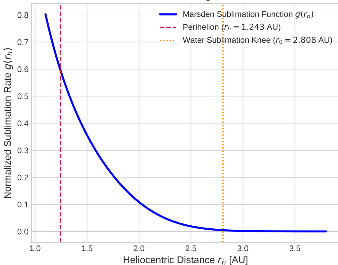
Model Choice: Sublimation Scaling vs Heliocentric Distance
