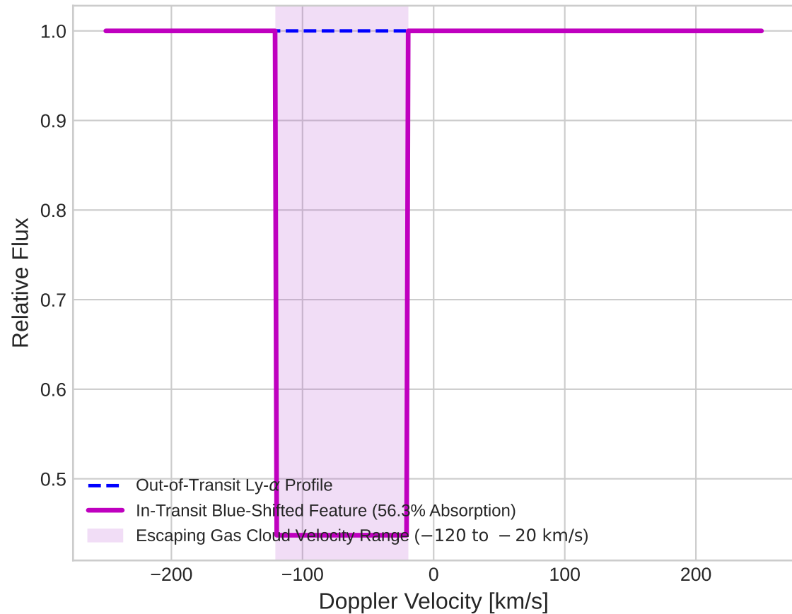
Giant Cloud Blue-Shifted Spectral Feature
