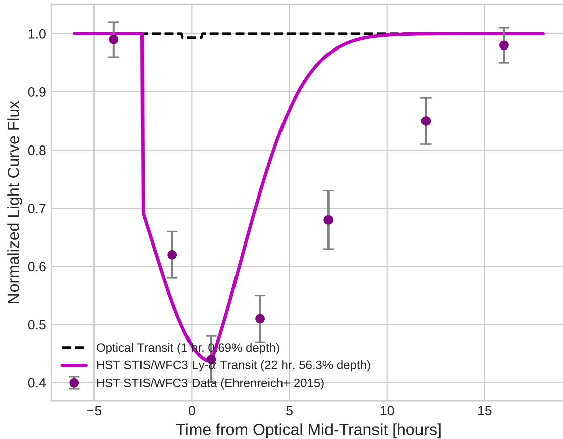
GJ 436b Asymmetric 22-Hour Ly-alpha Transit
