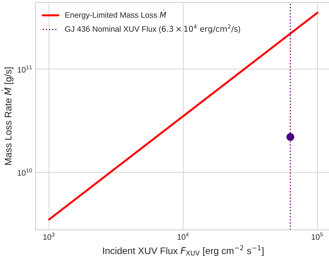
Model Choice: Mass Loss vs M-Dwarf XUV Flux
