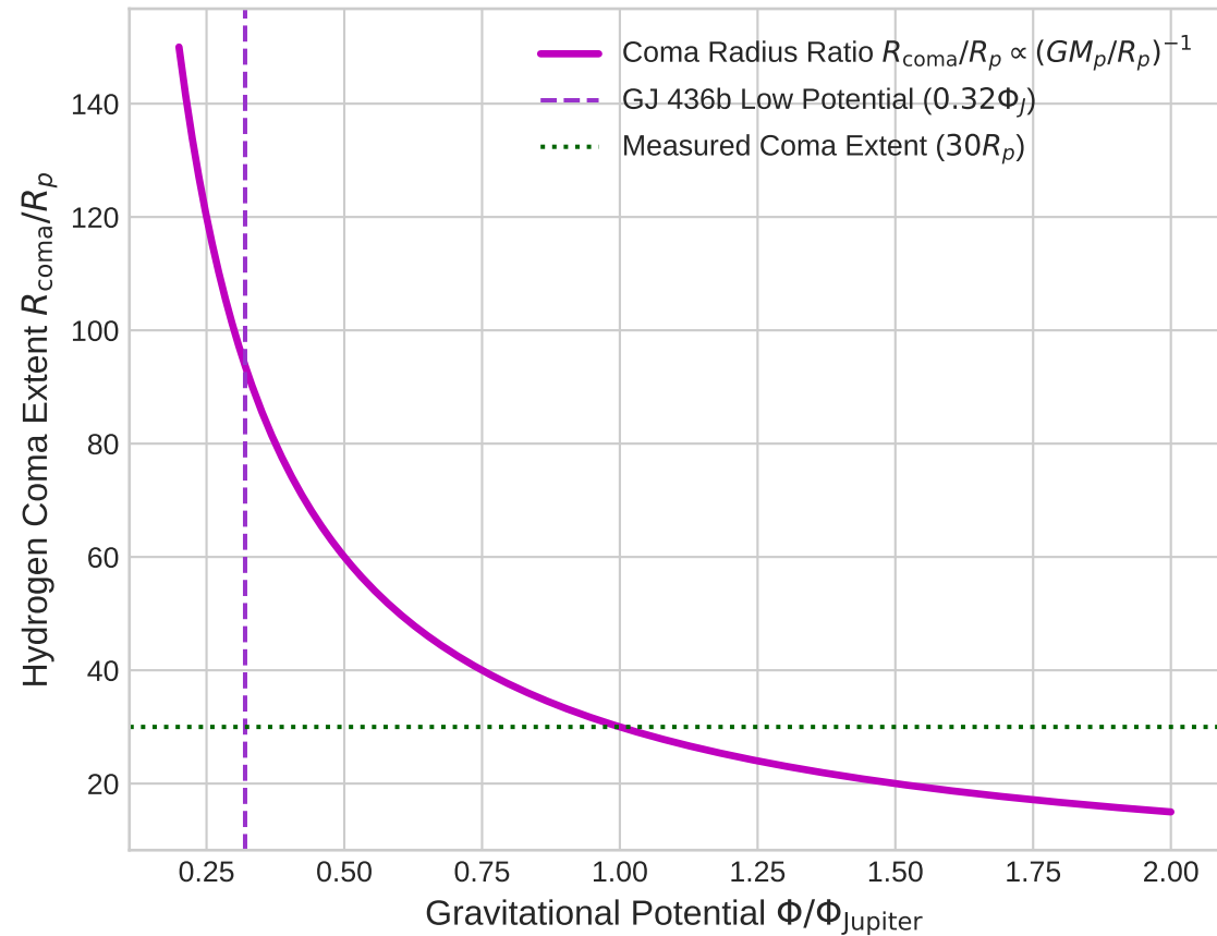
Model Choice: Low Potential Exospheric Expansion
