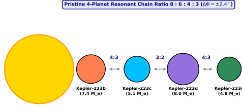
Physical Configuration Diagram: Kepler-223 Four-Planet Resonant Laplace Chain
