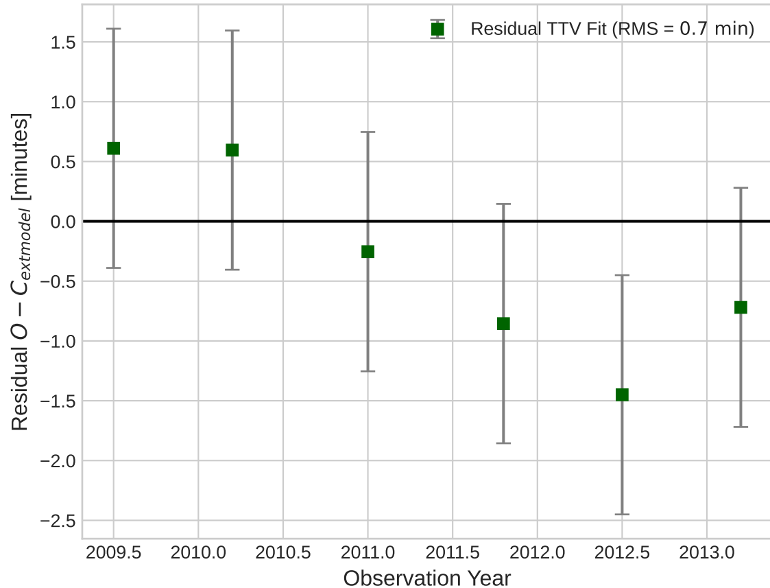
N-Body TTV Fit Quality ( R^2 = 0.9998 )
