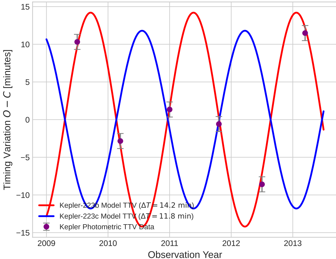
Kepler-223b & 223c Photometric TTV Ephemeris
