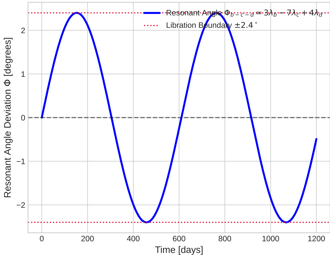
Model Choice: 3-Body Resonant Angle Libration
