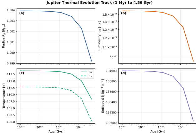
Figure 1: Scenario 1: 4-Panel diagnostic thermal cooling track for Jupiter ( M_p = 1.00 M_{\text{Jup}} , M_c = 12.0 M_{\oplus} , a = 5.204 \text{ AU} ) from t = 1 \text{ Myr} to 4.56 \text{ Gyr} .
