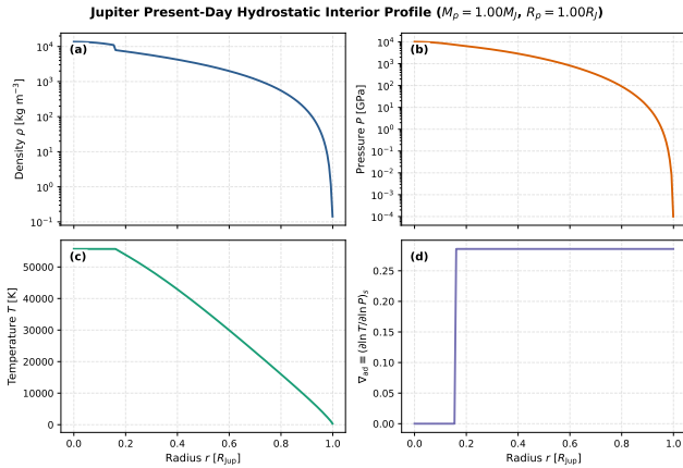
Figure 2: Scenario 1: 1D interior hydrostatic profile ( \rho, P, T, \nabla_{\text{ad}} ) of present-day Jupiter at 4.56 \text{ Gyr} , demonstrating smooth un-truncated radial coverage from core ( r/R_p = 0.00 ) to atmosphere (1.00).
