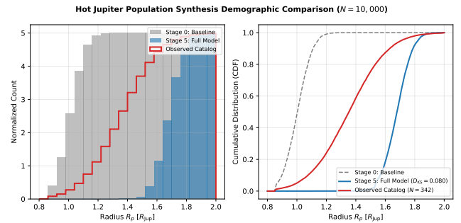
Figure 9: Scenario 8: Cumulative Distribution Function (CDF) and Kolmogorov-Smirnov (KS) metric comparison between baseline cooling models, interior heating models, and empirical exoplanet observations.
