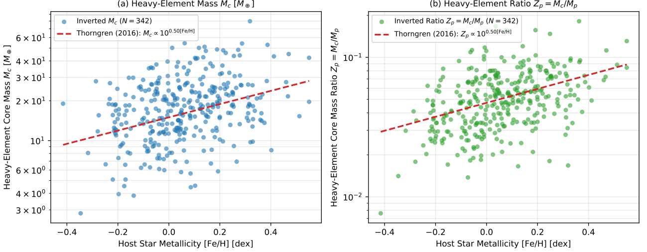
Figure 13: Dual-panel core mass inversion analysis across all N = 342 confirmed transiting Hot Jupiters: (a) Absolute heavy-element core mass M_c [ M_\oplus ] vs host star metallicity [Fe/H] [dex], and (b) Dimensionless heavy-element core mass fraction Z_p = M_c/M_p vs [Fe/H] [dex], compared against the empirical Thorngren et al. (2016) power-law trend.
