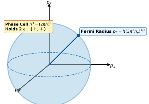
Figure 16: Fermi sphere momentum-space quantum state filling in metallic hydrogen.
