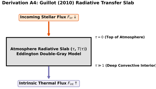
Figure 17: Two-stream double-gray radiative boundary geometry under stellar irradiation.
