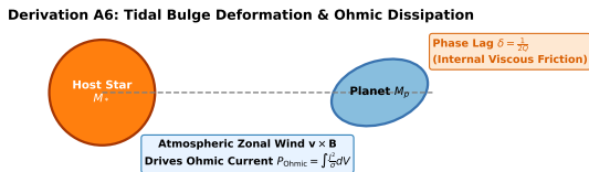
Figure 18: Quadrupolar tidal flexure and lagging tidal bulge geometry.
