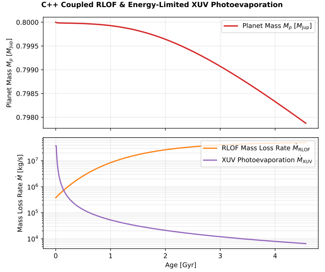
Figure 11: Scenario 10: Coupled planetary mass decay M_p(t) and mass loss rate components ( \dot{M}_{\text{RLOF}} vs \dot{M}_{\text{XUV}} ) over 4.56 Gyr.
