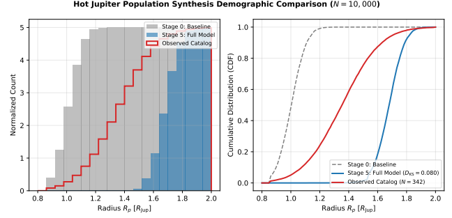
Figure 12: Probability density histogram (left) and Cumulative Distribution Function (right) tracking radius distribution progression across incremental stages (Stage 0 to Stage 5) against the full N = 342 confirmed NASA Exoplanet Archive Hot Jupiter catalog.
