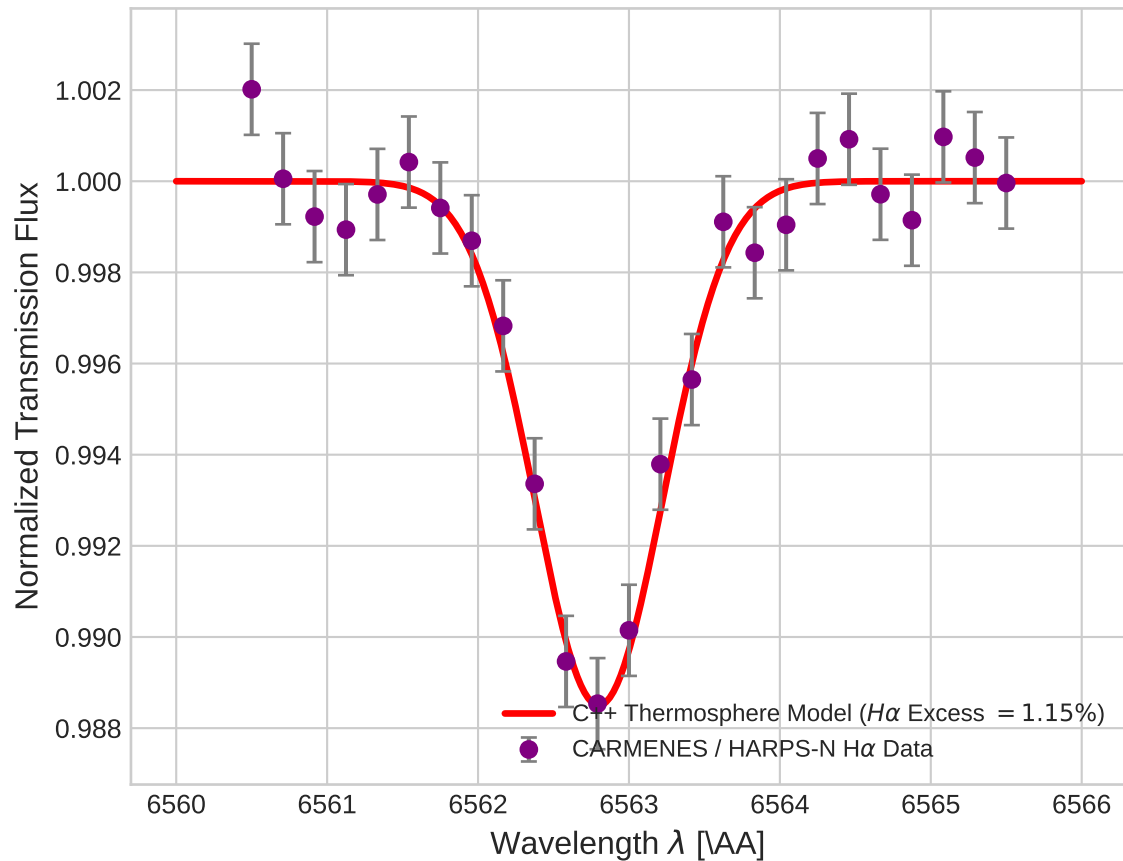
KELT-9b High-Res H\alpha Transmission Spectrum
