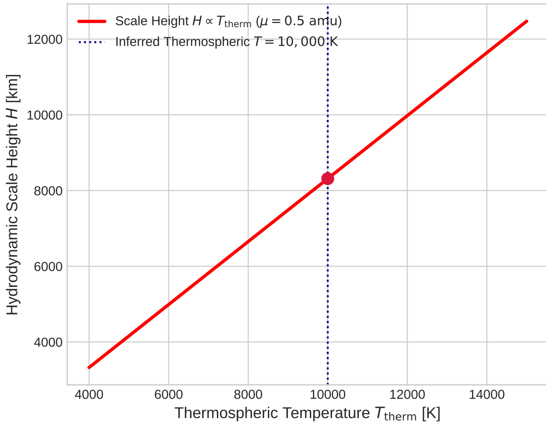
Model Choice: Scale Height vs Temperature
