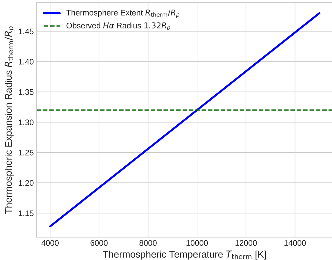
Model Choice: Atmospheric Expansion Scaling
