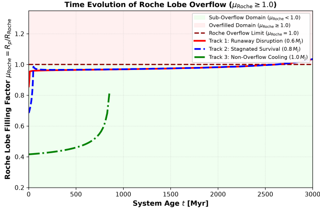
Figure 4: Roche Lobe Radius Contraction and Filling Factor. Time evolution of filling factor \mu_{\text{Roche}}(t) = R_p/R_{\text{Roche}} . Overfilling ( \mu_{\text{Roche}} \geq 1.0 , red shaded region) initiates hydrodynamic mass loss, while sub-overflow ( \mu_{\text{Roche}} < 1.0 , green shaded region) represents stable cooling.
