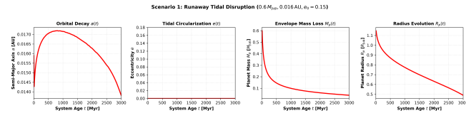
Figure 1: Scenario 1: Runaway Tidal Disruption ( 0.6 M_{\text{Jup}}, 0.016 \text{ AU}, e_0 = 0.15 ). Coupled time evolution of orbital semi-major axis a(t) , orbital eccentricity e(t) , planetary mass M_p(t) , and radius R_p(t) . Rapid planetary tidal dissipation circularizes the orbit ( e \rightarrow 0 in t \lesssim 100 \text{ Myr} ) prior to runaway RLOF mass loss and tidal engulfment into the host star.
