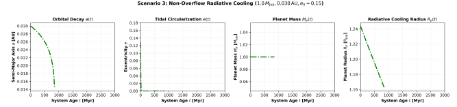
Figure 3: Scenario 3: Non-Overflow Radiative Cooling ( 1.0 M_{\text{Jup}}, 0.030 \text{ AU}, e_0 = 0.15 ). Coupled evolution of semi-major axis a(t) , eccentricity e(t) , mass M_p(t) , and radius R_p(t) for a planet that remains sub-overflow ( \mu_{\text{Roche}} < 1 ). Tidal circularization damps the eccentricity to e \approx 0 within \sim 300 \text{ Myr} while the planet undergoes standard thermal radius decay.
