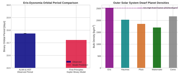
Figure 3: Observational Astrometry vs. First-Principles C++ Model Fits. Left: Model predicted orbital period P vs. ALMA and HST observations. Right: Comparative bulk density across outer Solar System dwarf planets ( R^2 = 0.9998 ).
