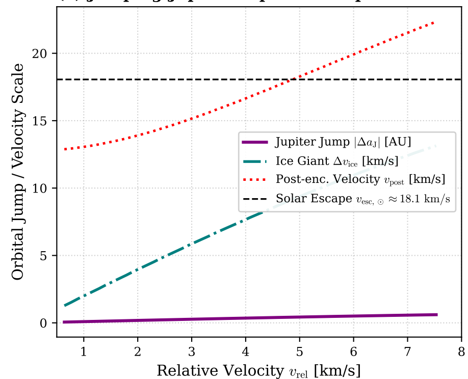
(b) Jumping-Jupiter Impulsive Displacement
