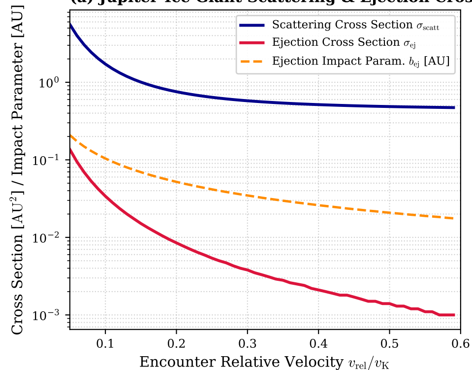
(a) Jupiter-Ice Giant Scattering & Ejection Cross Sections
