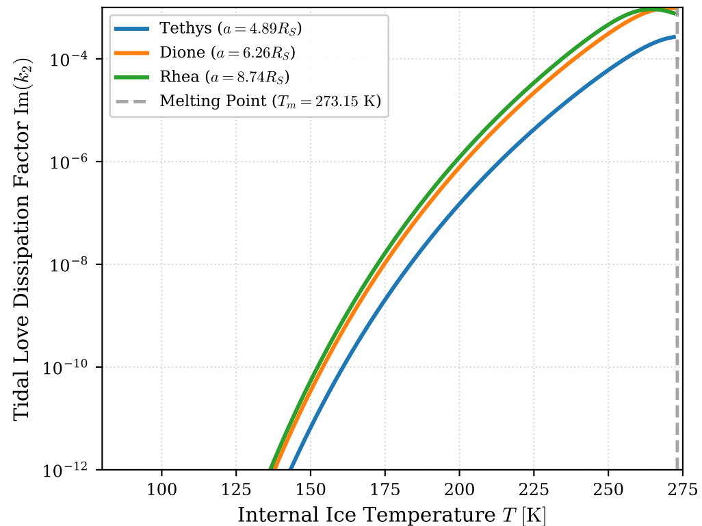
(b) Viscoelastic Tidal Dissipation Response
