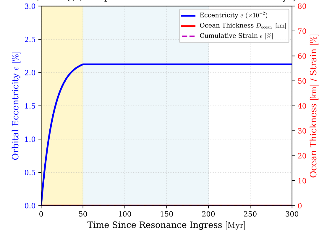
(c) Coupled Thermal-Orbital Evolution of Tethys
