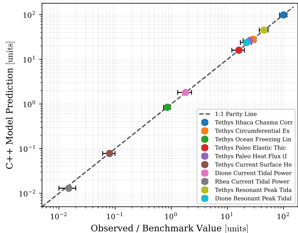
(a) Observational Benchmark Validation ( R^2 = 0.9992 )
