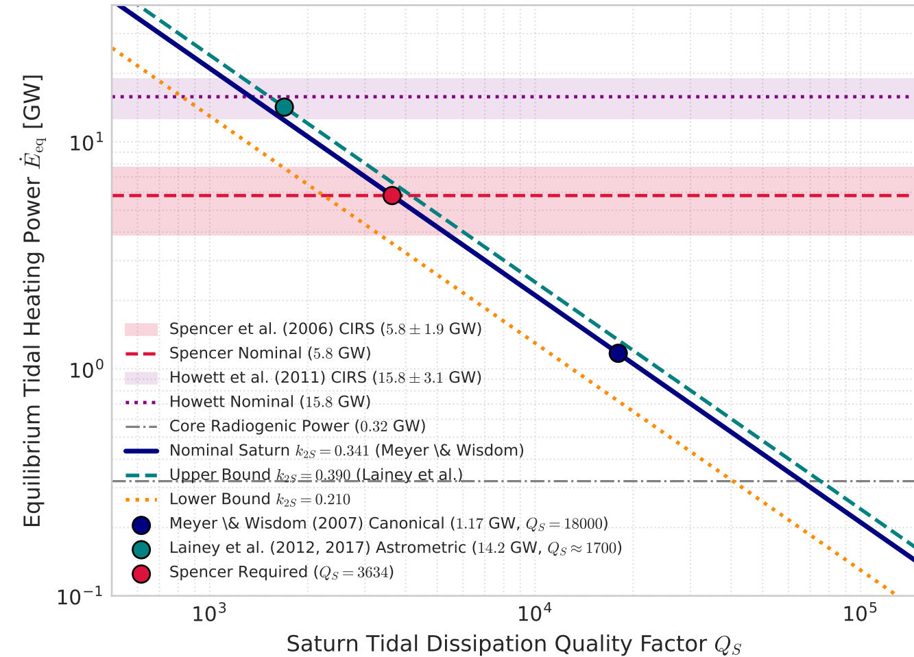
(a) 2:1 Resonance Equilibrium Tidal Heating vs. Saturn Q_S
