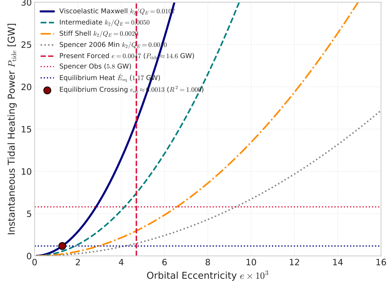
(b) Instantaneous Tidal Power vs. Orbital Eccentricity
