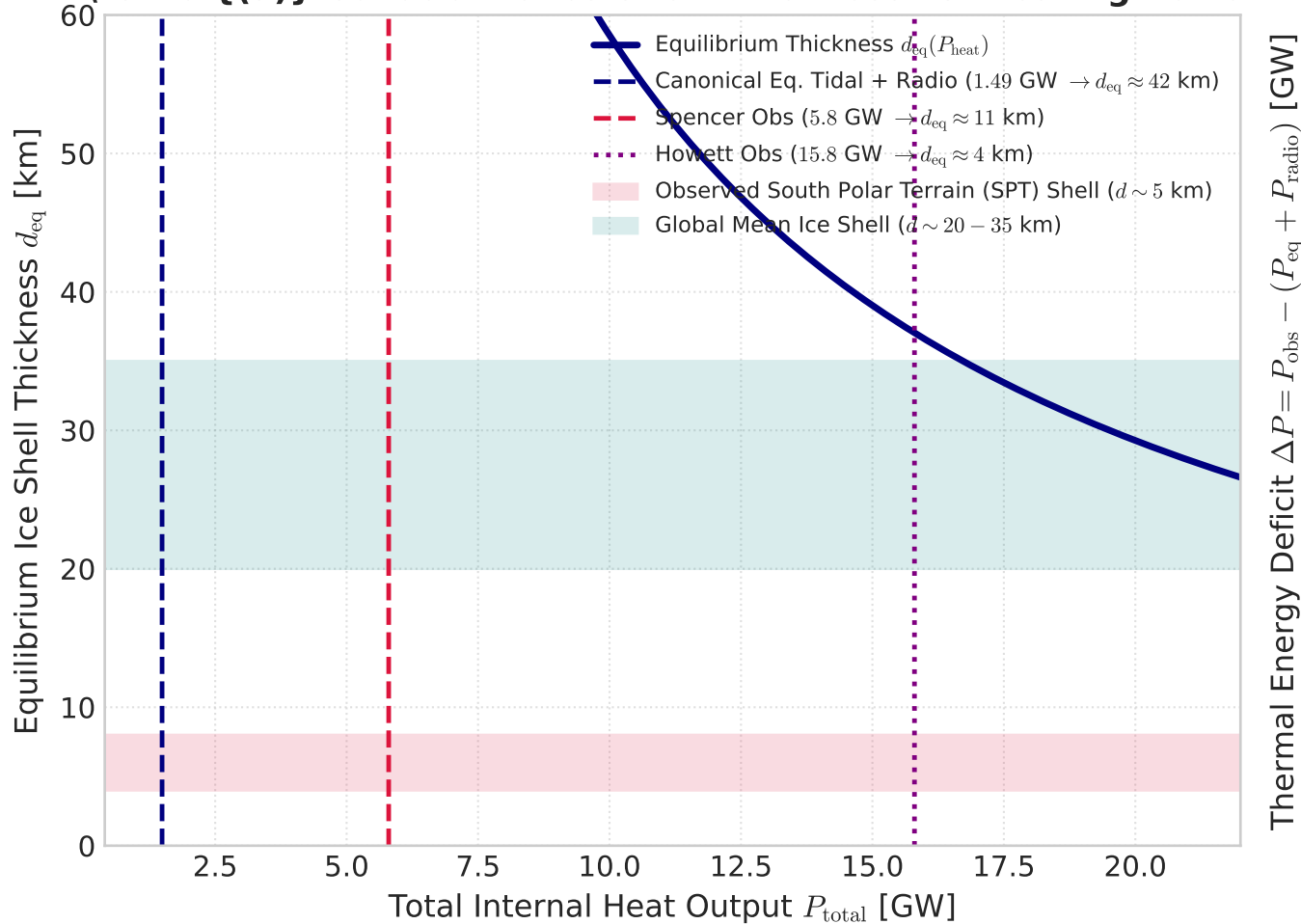
(a) Conductive Ice Shell Thickness vs. Heating Power
