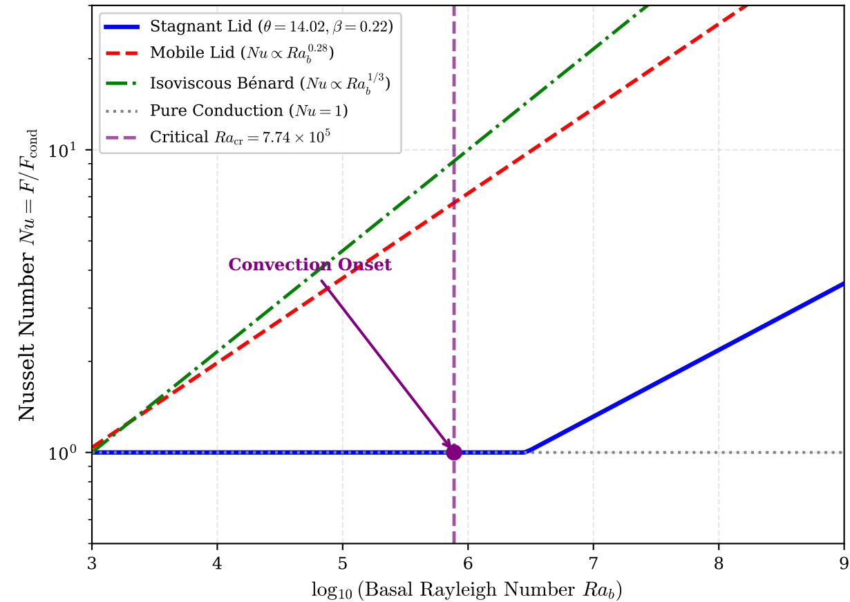
(a) Heat Transfer Scaling: Stagnant Lid vs. Mobile Lid
