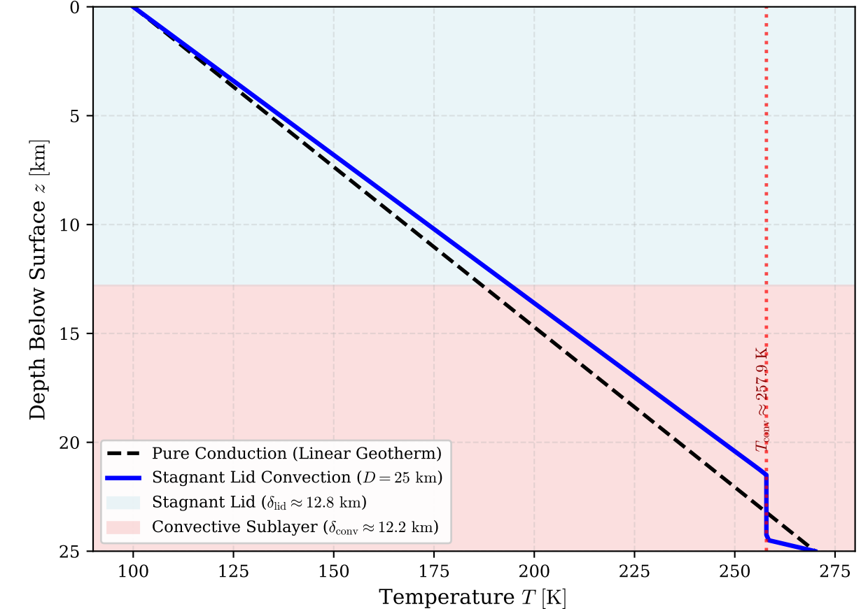
(c) Ice Shell Thermal Geotherms
