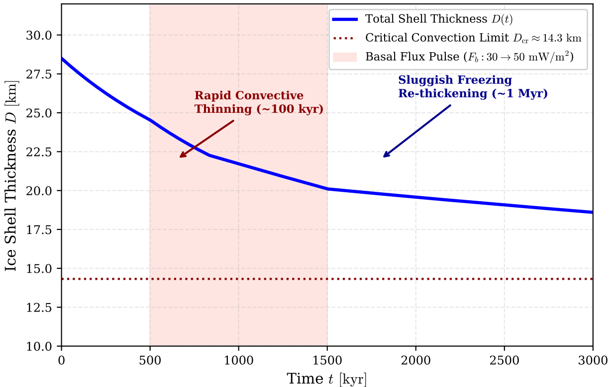
(a) Transient Response to Basal Heat Flux Step
