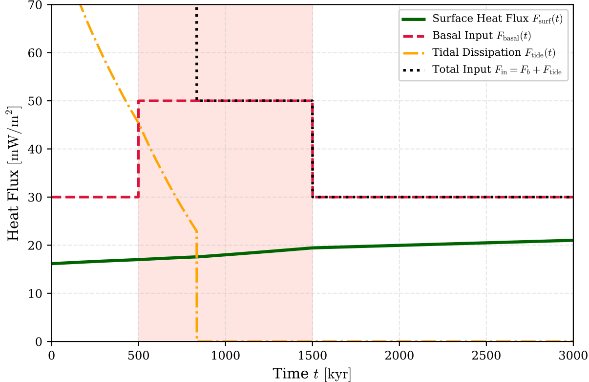
(c) Dynamic Energy Balance at Ice-Ocean Boundary
