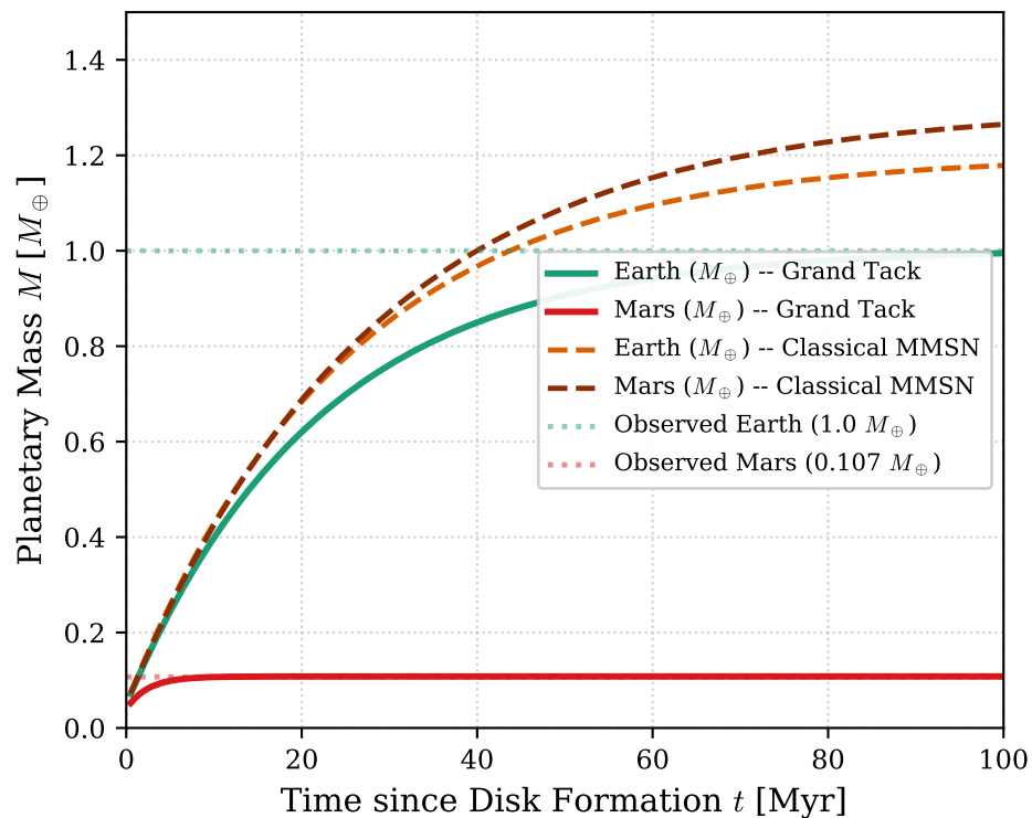
(a) Accretion Mass Growth: Mars Problem Resolution
