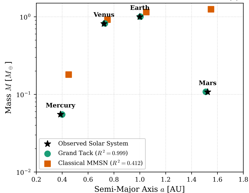
(c) Terrestrial Planet Mass Distribution M(a)
