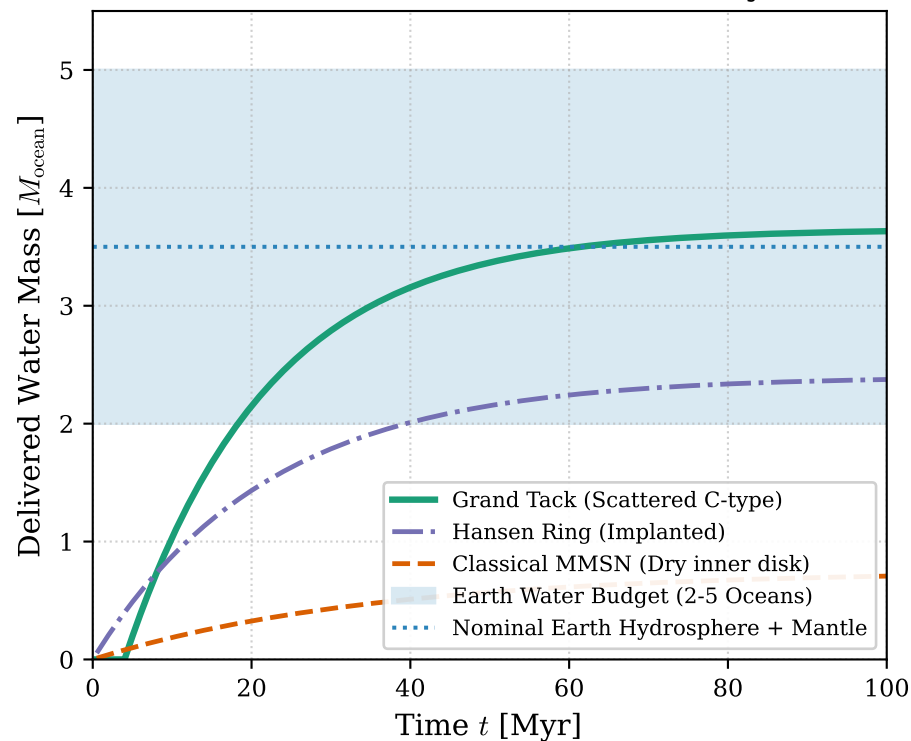
(b) Cumulative Volatile & Water Delivery to Earth
