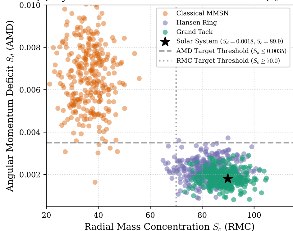
(c) Dynamical Excitation vs Concentration ( S_d - S_c )
