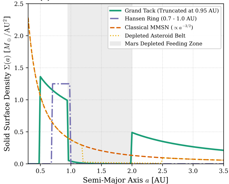
(a) Primordial Planetesimal Disk Profiles
