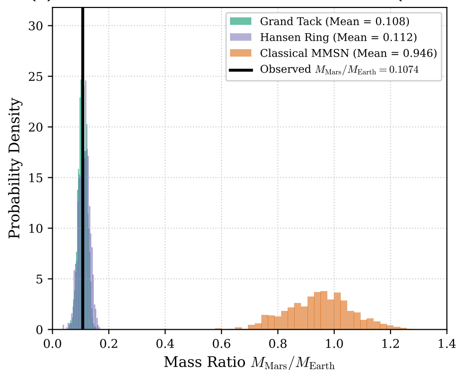
(b) Mars-to-Earth Mass Ratio Distribution ( N = 1000 )
