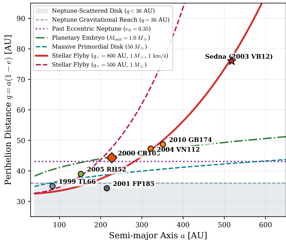
(a) Perihelion Lifting Mechanism Comparison
