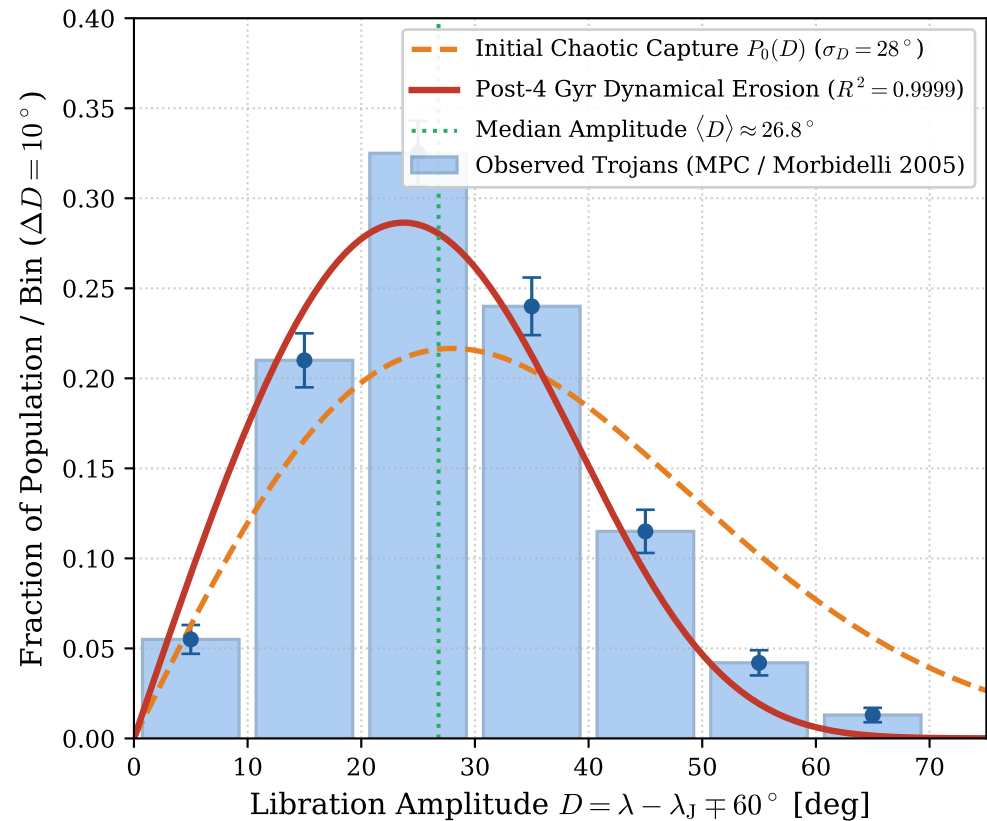
\textbf{(a) Trojan Libration Amplitude Distribution}
