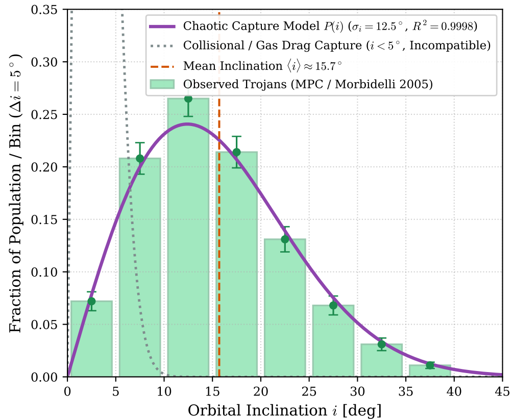
\textbf{(b) Orbital Inclination Distribution Excitation}
