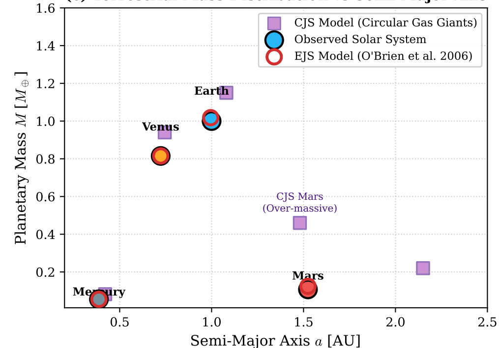
(c) Terrestrial Mass Distribution vs Semi-Major Axis
