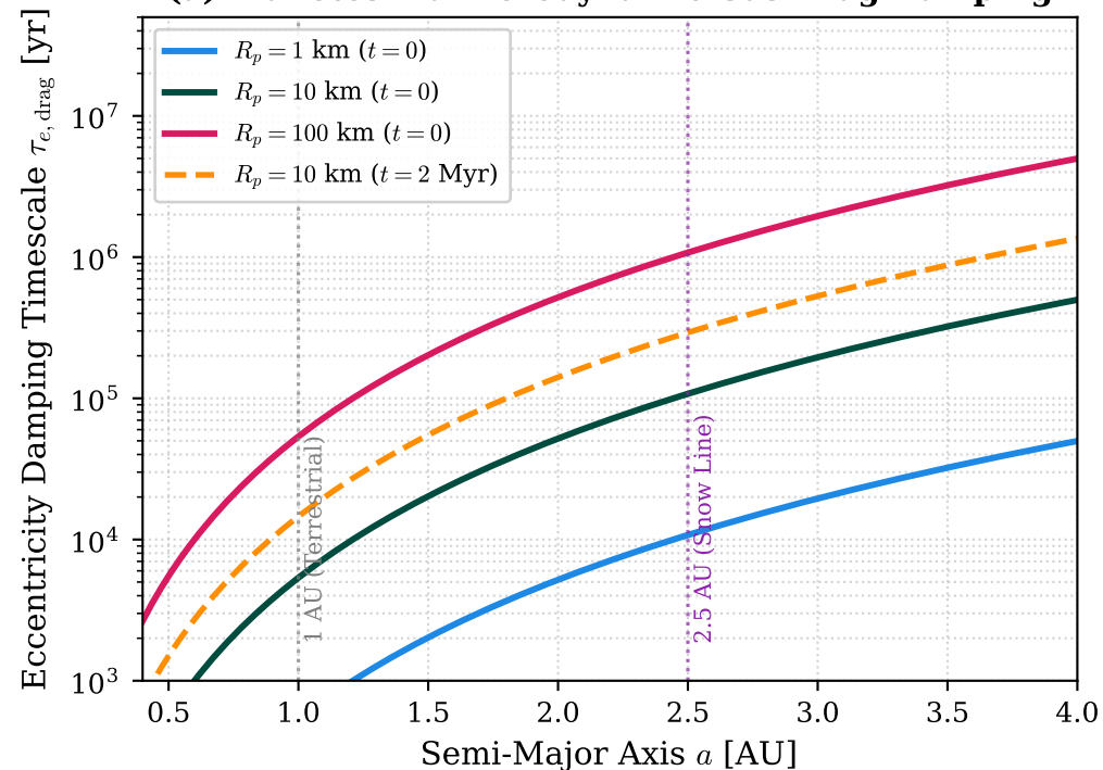
(a) Planetesimal Aerodynamic Gas Drag Damping
