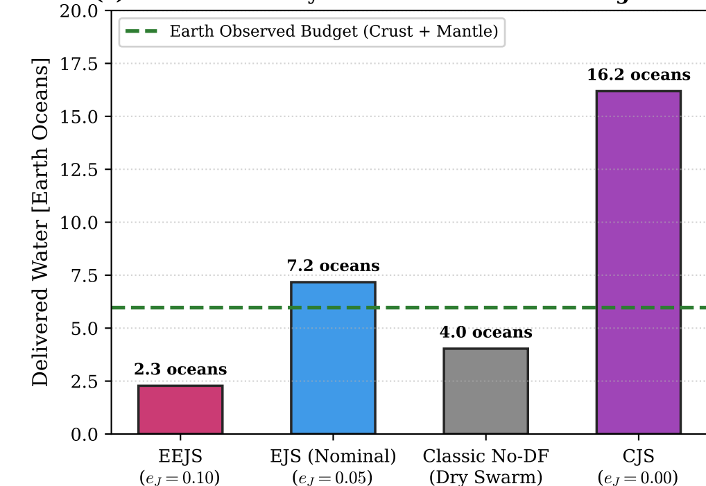
(c) Volatile Delivery across Giant Planet Configurations
