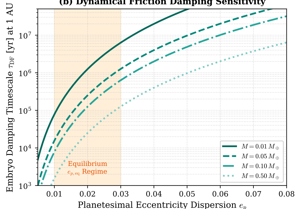
(b) Dynamical Friction Damping Sensitivity
