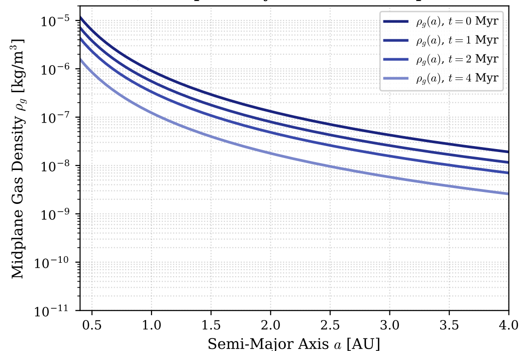
(a) Protoplanetary Nebula Gas Dissipation
