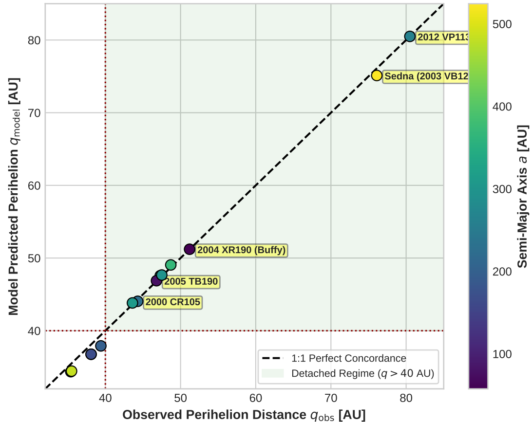
(b) Observed vs. Secular Model ( R^2 = 0.9962 )
