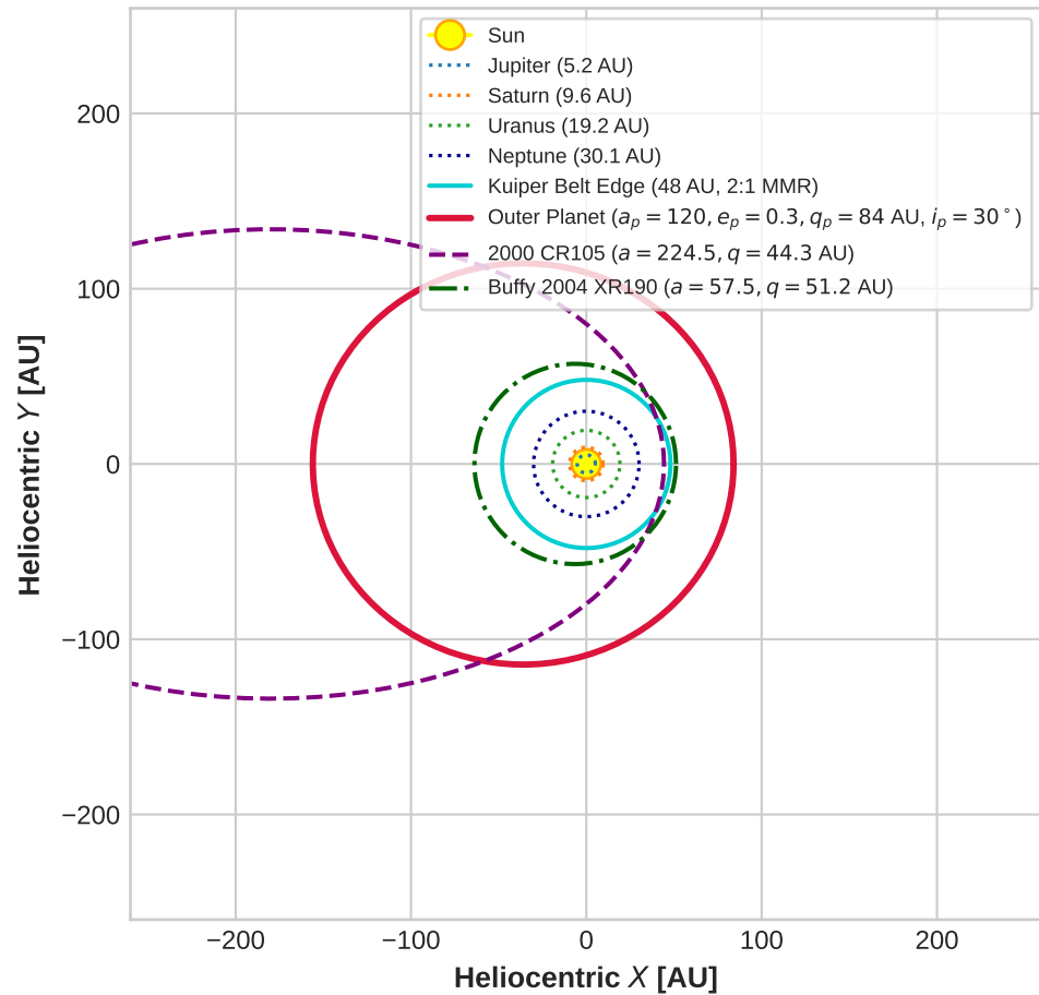
(a) Outer Solar System & Detached Belt Architecture
