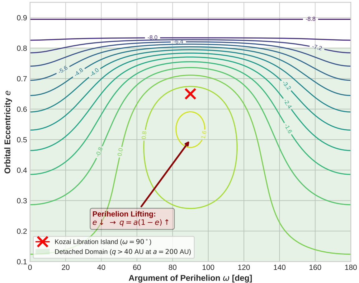
(b) Kozai-Lidov Secular Resonance Phase Space
