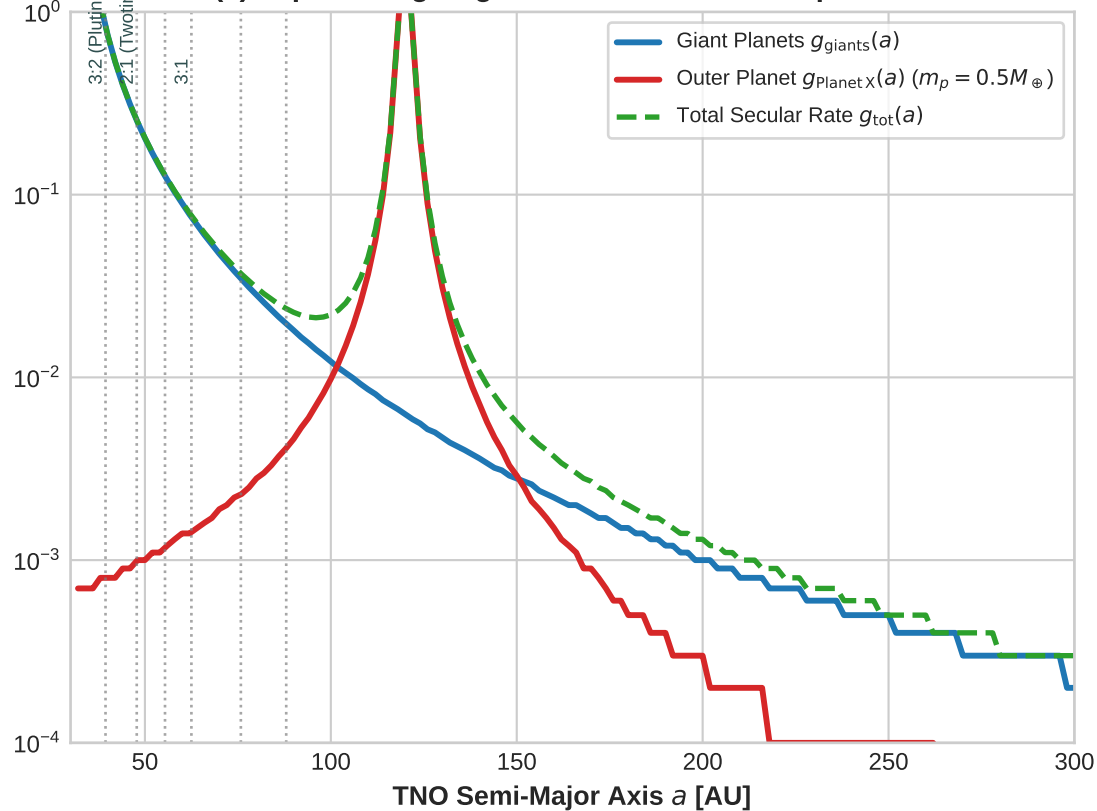
(a) Laplace-Lagrange Secular Precession Spectrum
