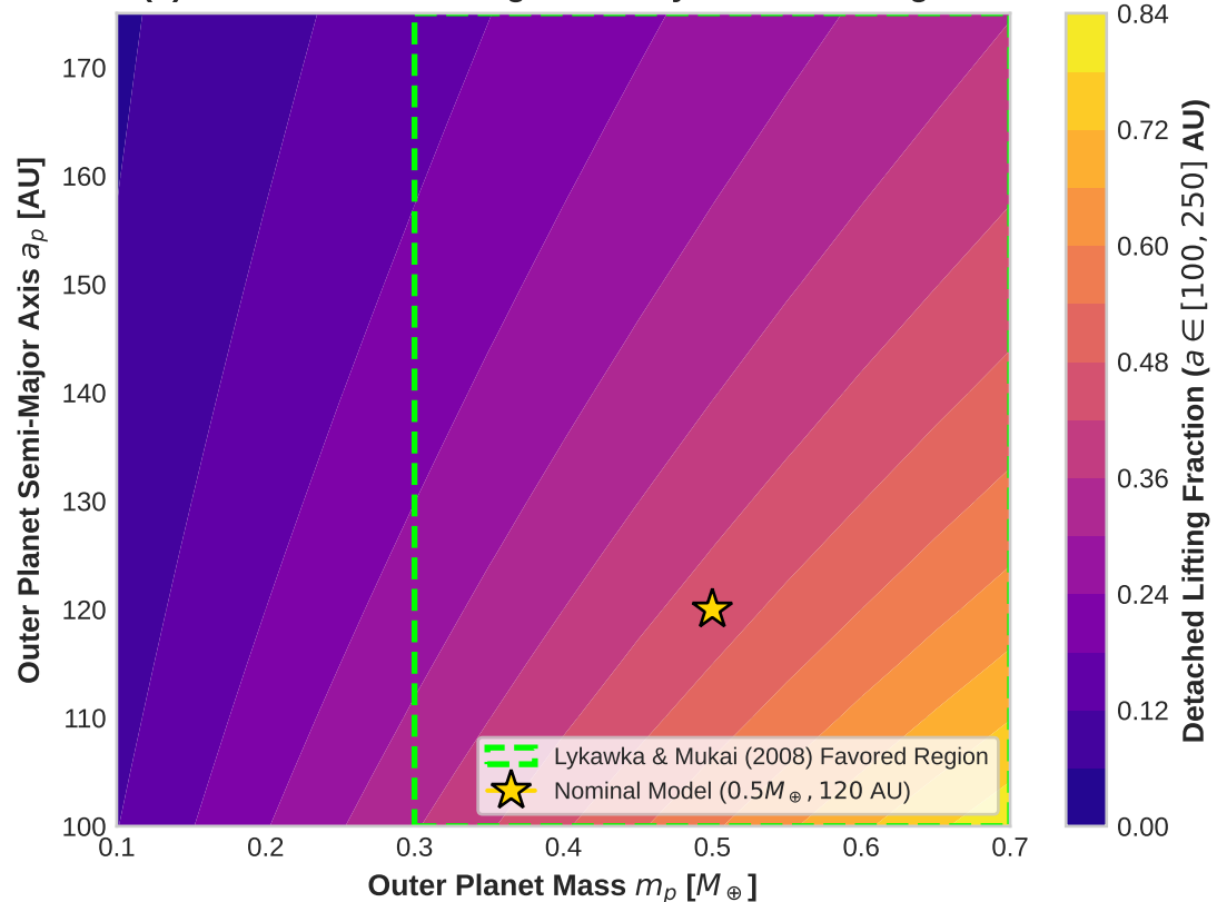
(b) Detached Disk Lifting Efficiency & Favored Regime
