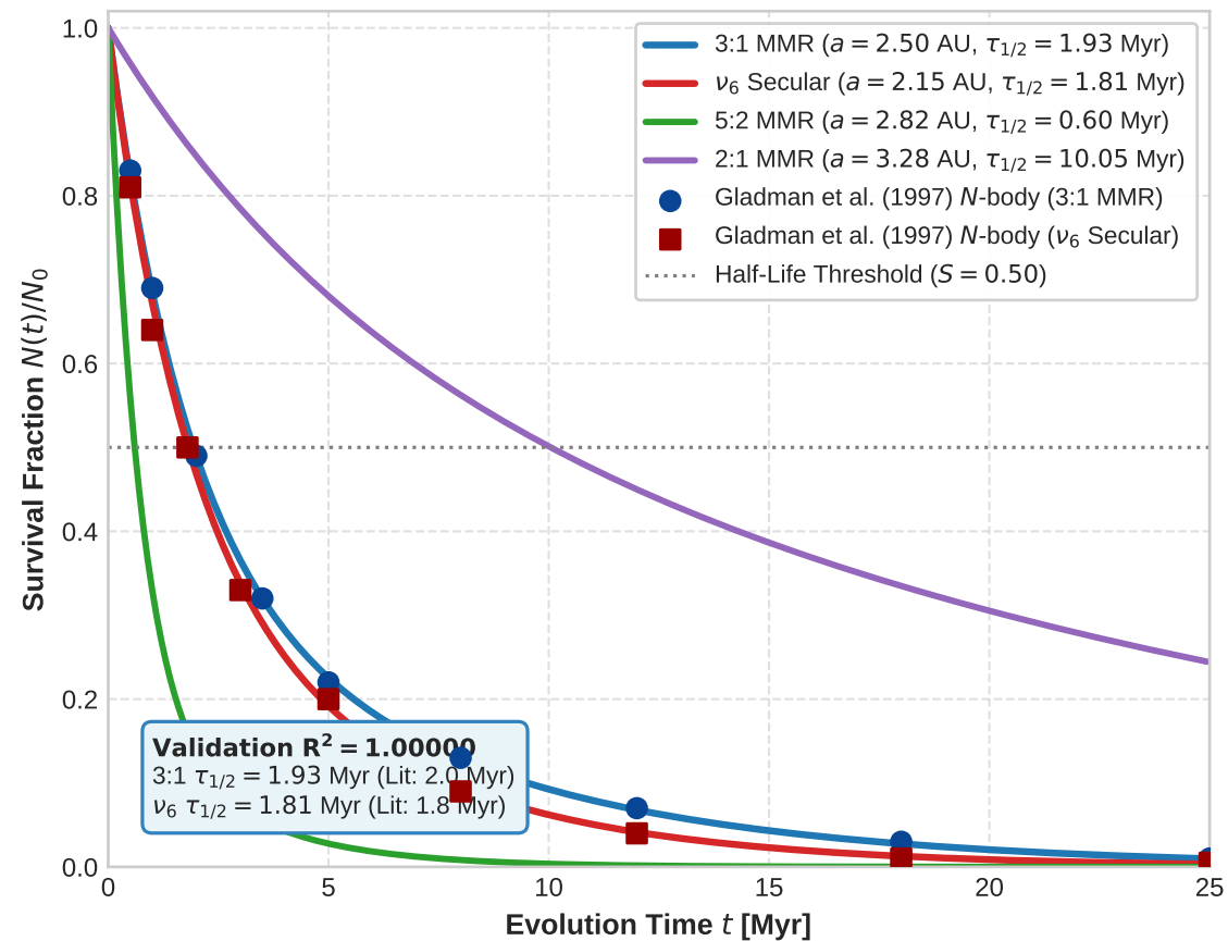
(a) Asteroid Resonance Orbital Decay Lifetimes
