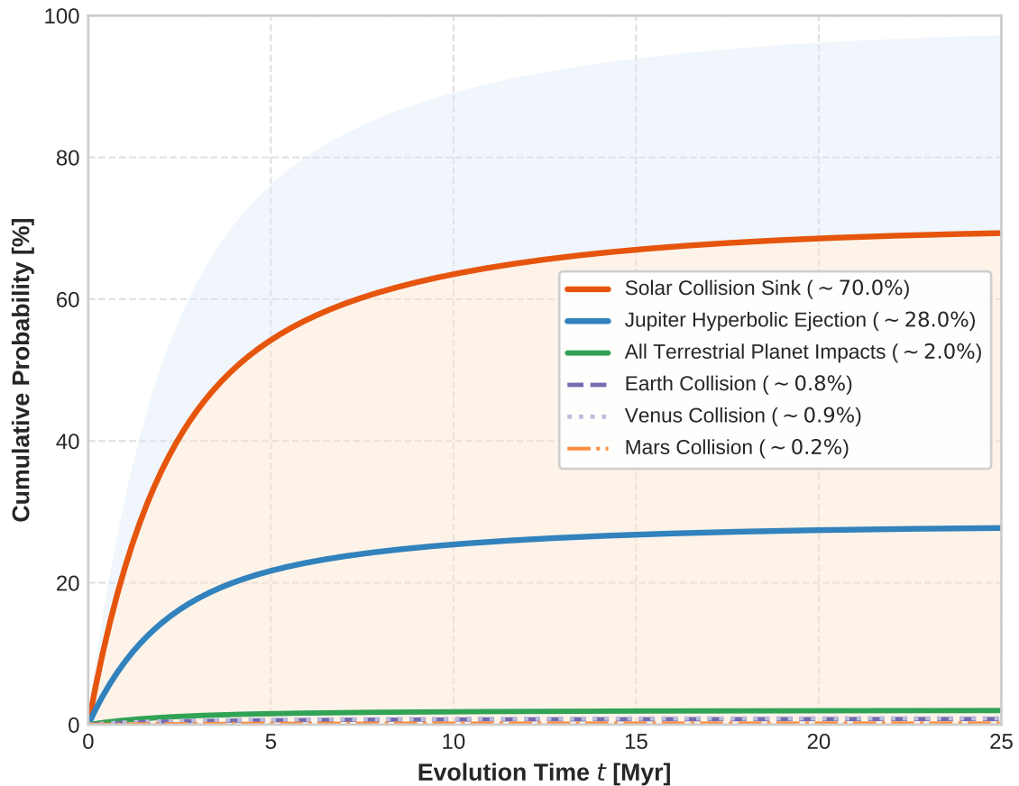
(b) 3:1 MMR Cumulative Elimination Fates
