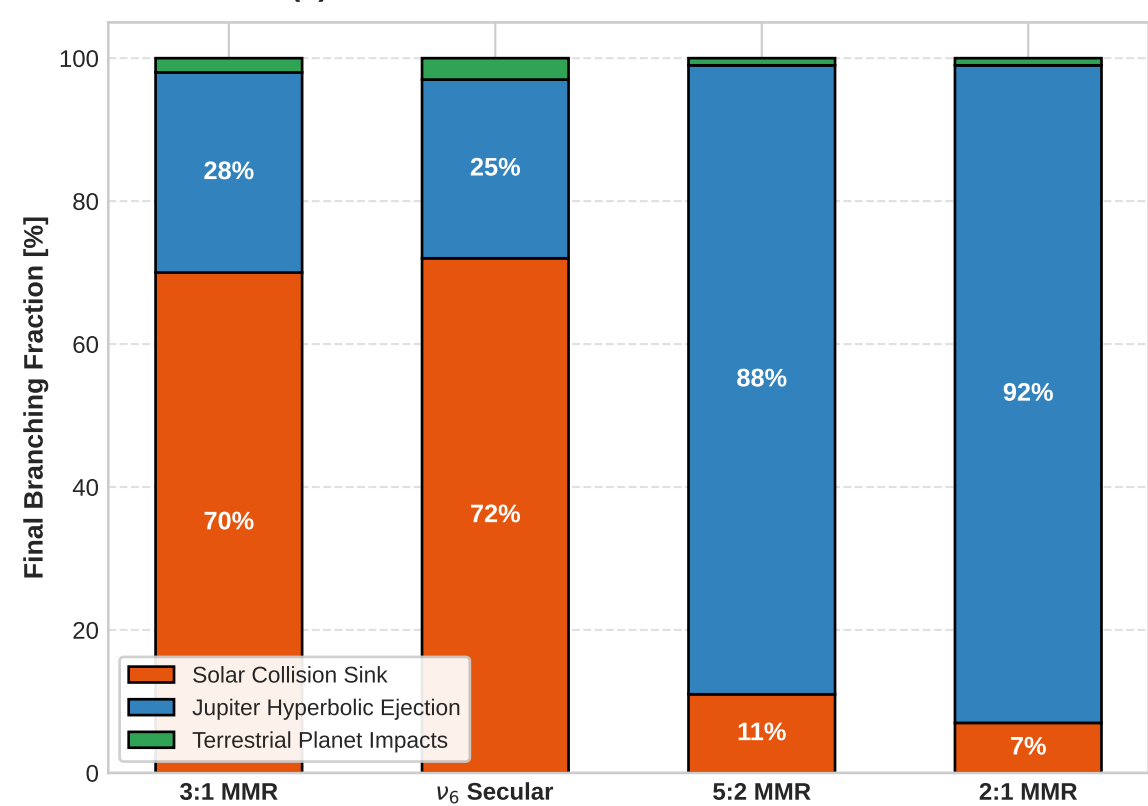
(d) Ultimate Sinks Across Main-Belt Resonances
