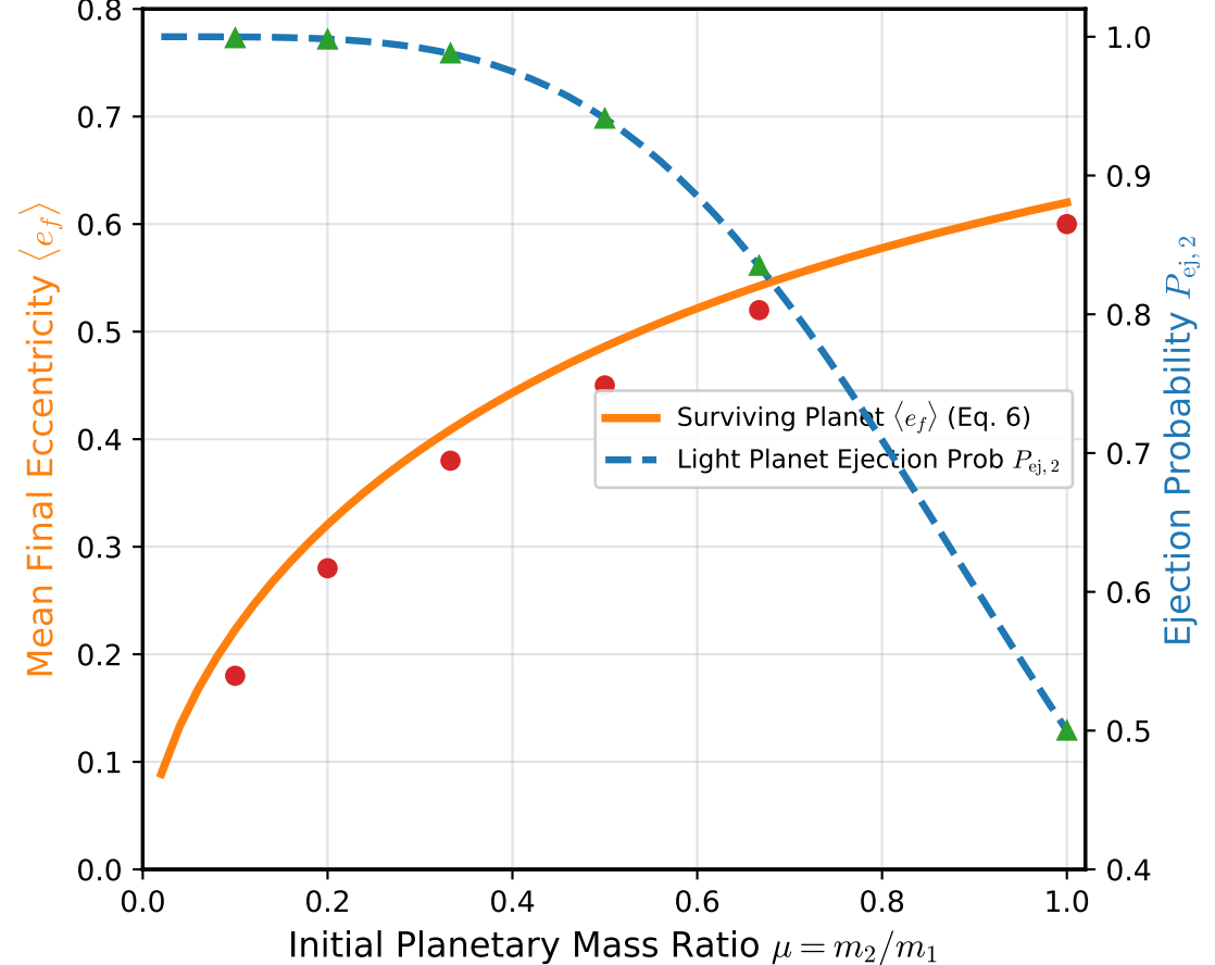
(c) Mass Hierarchy & Ejection Kinetics
