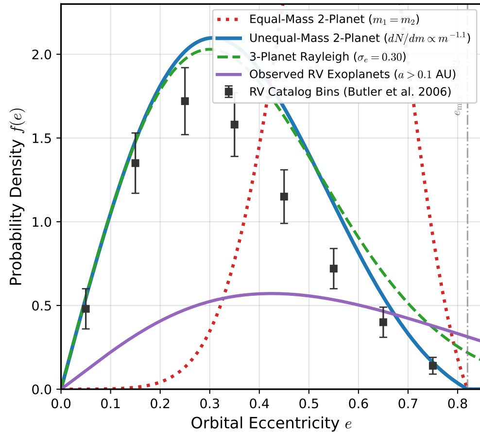
(a) Post-Scattering Eccentricity PDF
