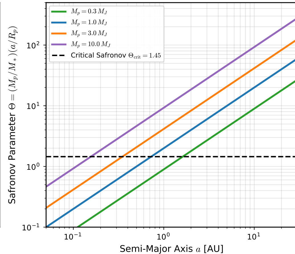
(b) Safronov Scattering Energetics
