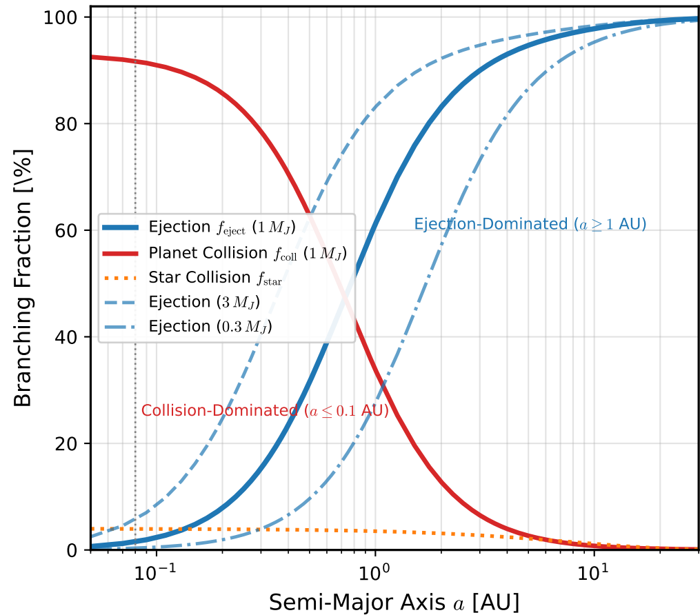
(a) Outcome Branching Ratios vs Semi-Major Axis
