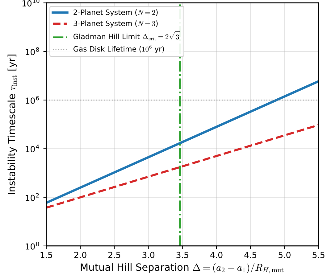
(c) Instability Timescale Scaling
