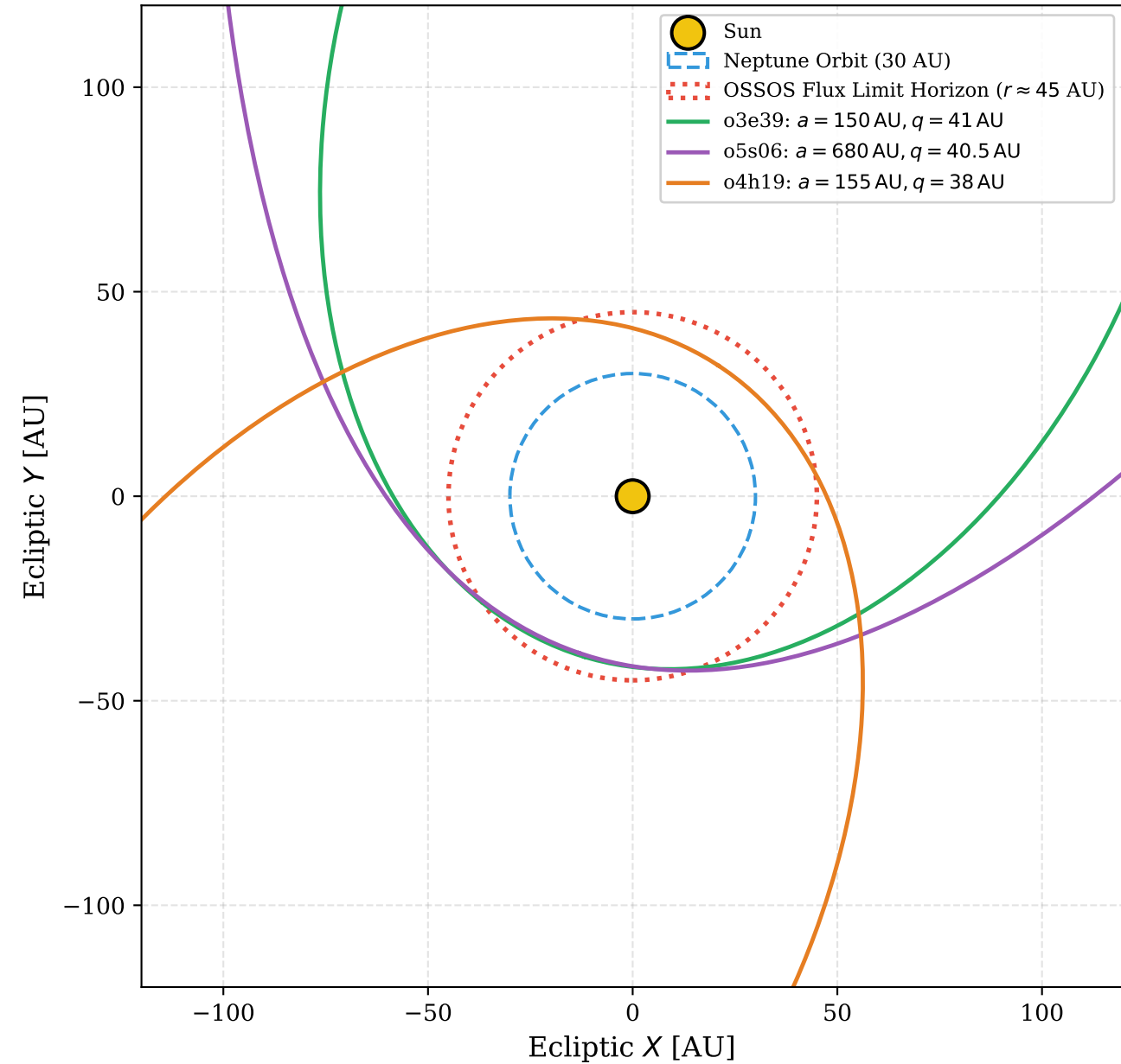
(b) Detection Horizon & Perihelion Crossing
