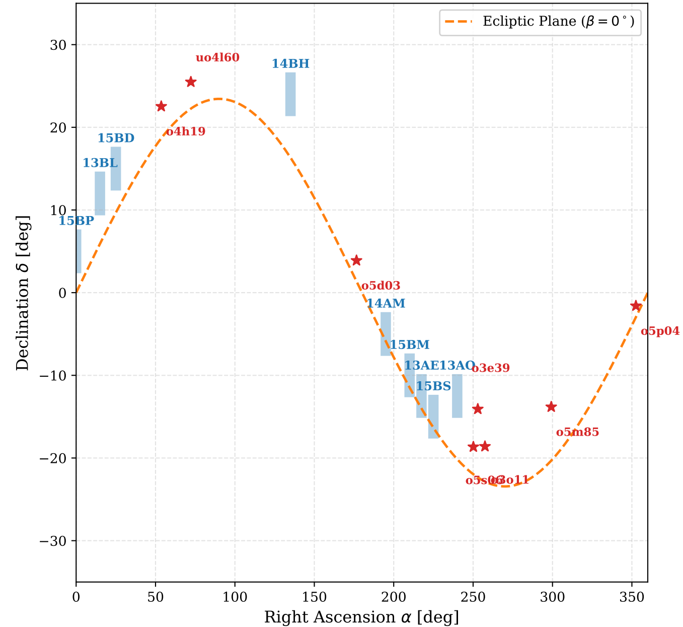
(a) OSSOS Sky Coverage Footprint & Discoveries
