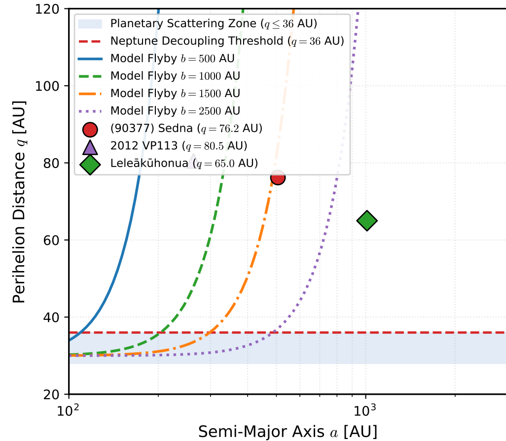
(c) Perihelion Lifting in (a, q) Phase Space
