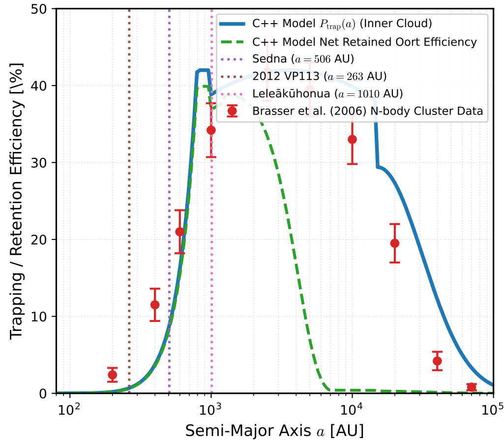
(a) Oort Cloud Trapping Efficiency vs a
