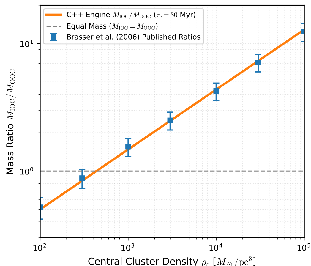
(b) Mass Ratio M_{\text{IOC}}/M_{\text{OOC}} vs \rho_c
