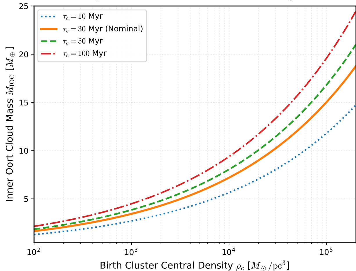
(c) Sedna Sphere Mass M_{\text{IOC}} vs Cluster Density & Lifetime
