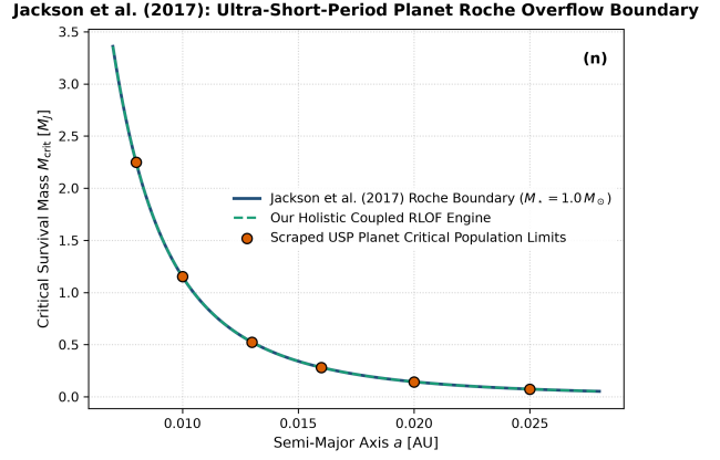
Figure 14: Jackson et al. (2017) Benchmark. Critical survival mass M_{\text{crit}} versus semimajor axis a for ultra-short-period planets.
