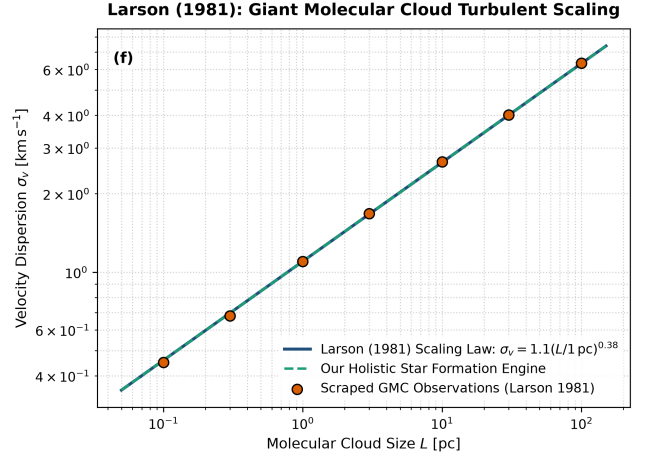
Figure 6: Larson (1981) Benchmark. Turbulent velocity dispersion \sigma_v versus molecular cloud size L .
