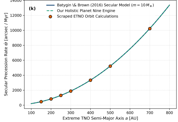
Batygin & Brown (2016): Planet Nine Secular Perihelion Shepherding
