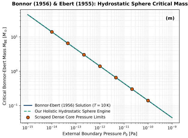
Figure 13: Bonnor-Ebert Benchmark. Maximum stable sphere mass M_{BE} versus ambient boundary pressure P_0 .
