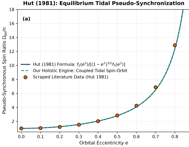
Figure 1: Hut (1981) Benchmark. Pseudo-synchronous spin ratio \Omega_{\text{ps}}/n versus orbital eccentricity e , comparing Hut’s analytical formula, scraped literature points, and our holistic multi-physics engine.
