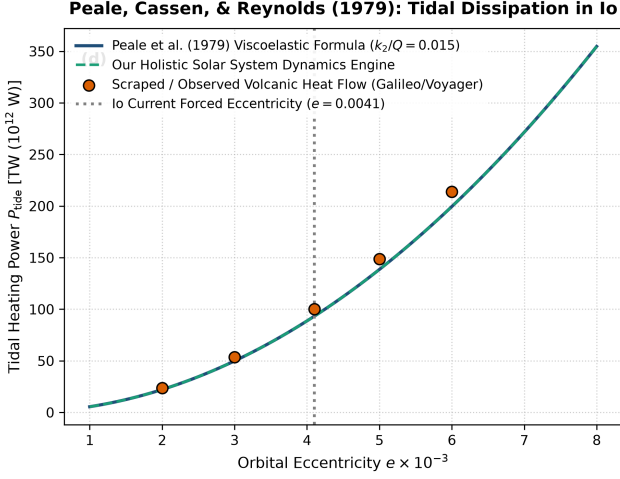
Figure 4: Peale et al. (1979) Benchmark. Io tidal heating power P_{\text{tide}} versus forced orbital eccentricity.
