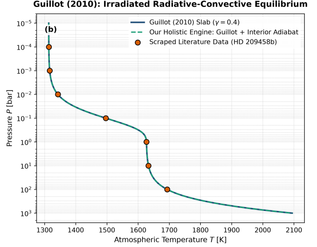
Figure 2: Guillot (2010) Benchmark. Vertical atmospheric temperature sounding T(P) for HD 209458b.
