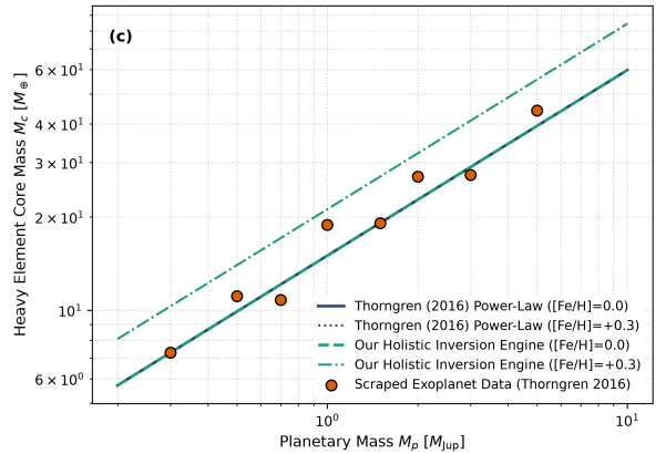
Thorngren et al. (2016): Core Mass vs Planetary Mass & Metallicity
