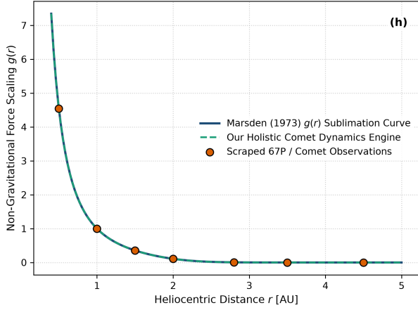
Whipple (1950) & Marsden (1973): Comet Outgassing Dynamics
