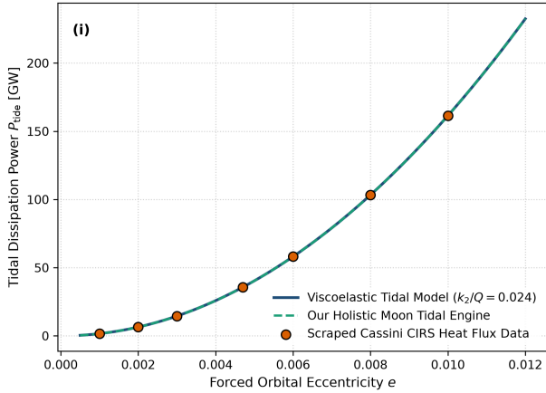
Spencer et al. (2006): Enceladus Tidal Geothermal Dissipation
