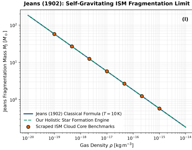
Figure 12: Jeans (1902) Benchmark. Critical Jeans fragmentation mass M_J versus interstellar gas density \rho .
