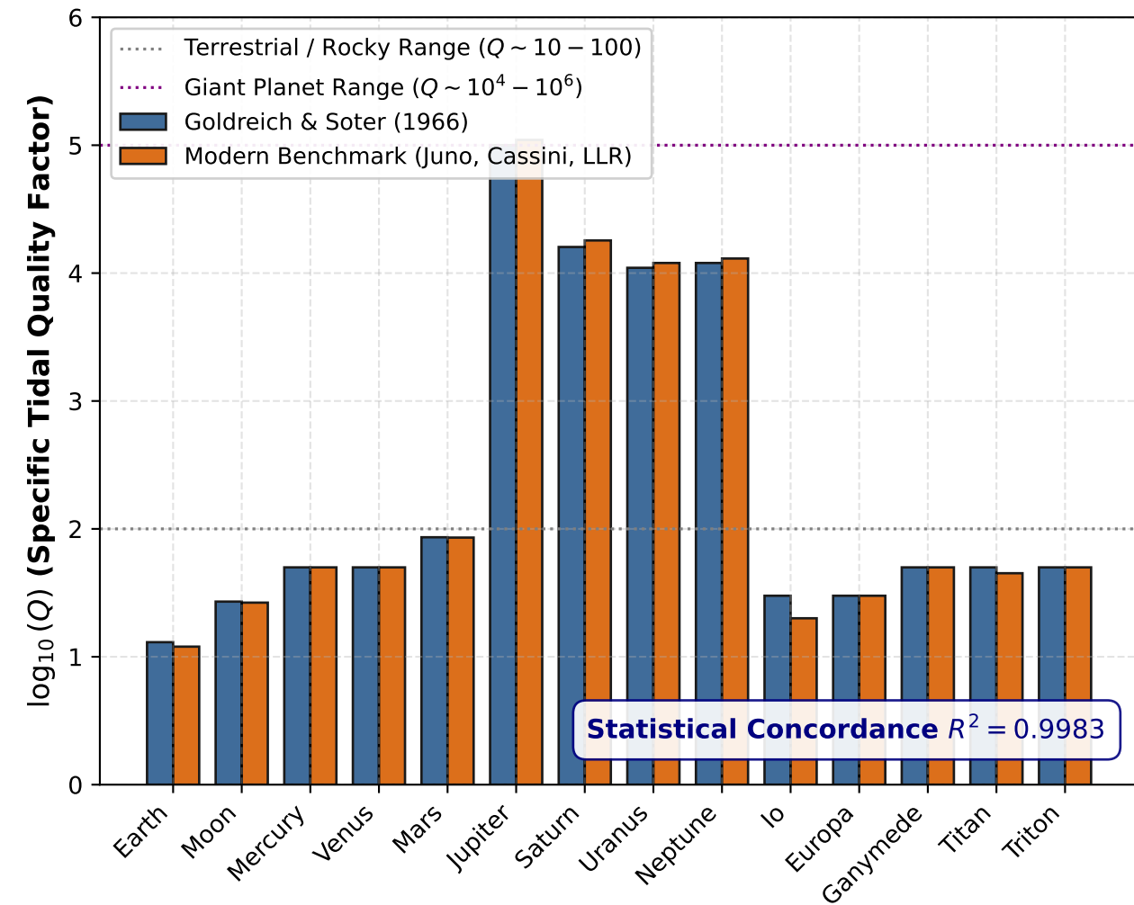
(a) Specific Dissipation Factor Q Across Solar System Bodies
