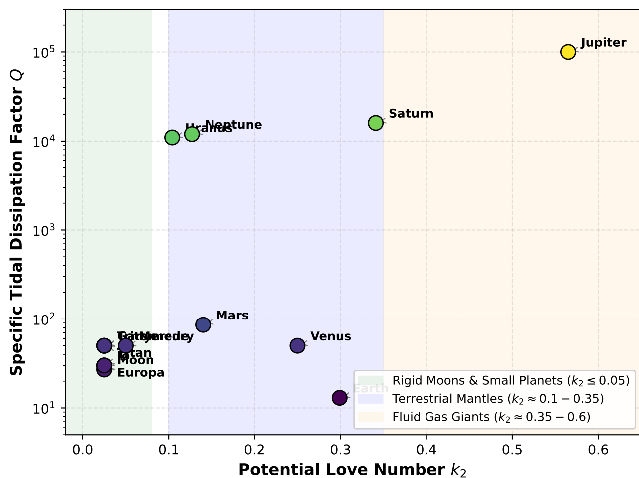
(b) Elastic/Fluid Rigidity ( k_2 ) vs Dissipation ( Q )
