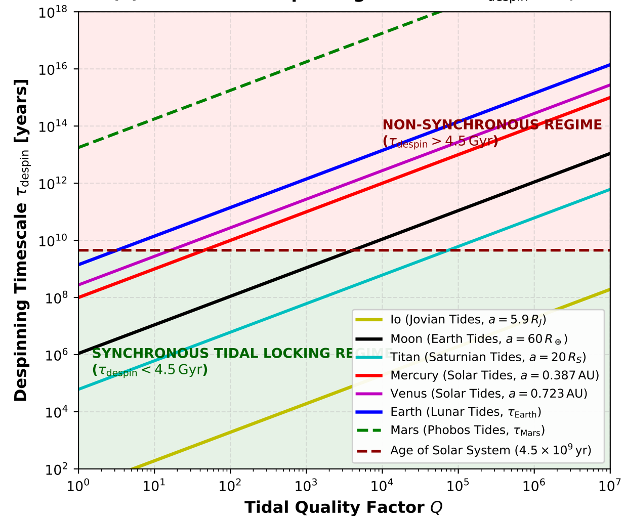
(a) Rotational Despinning Timescale \tau_{\text{despin}} vs Q
