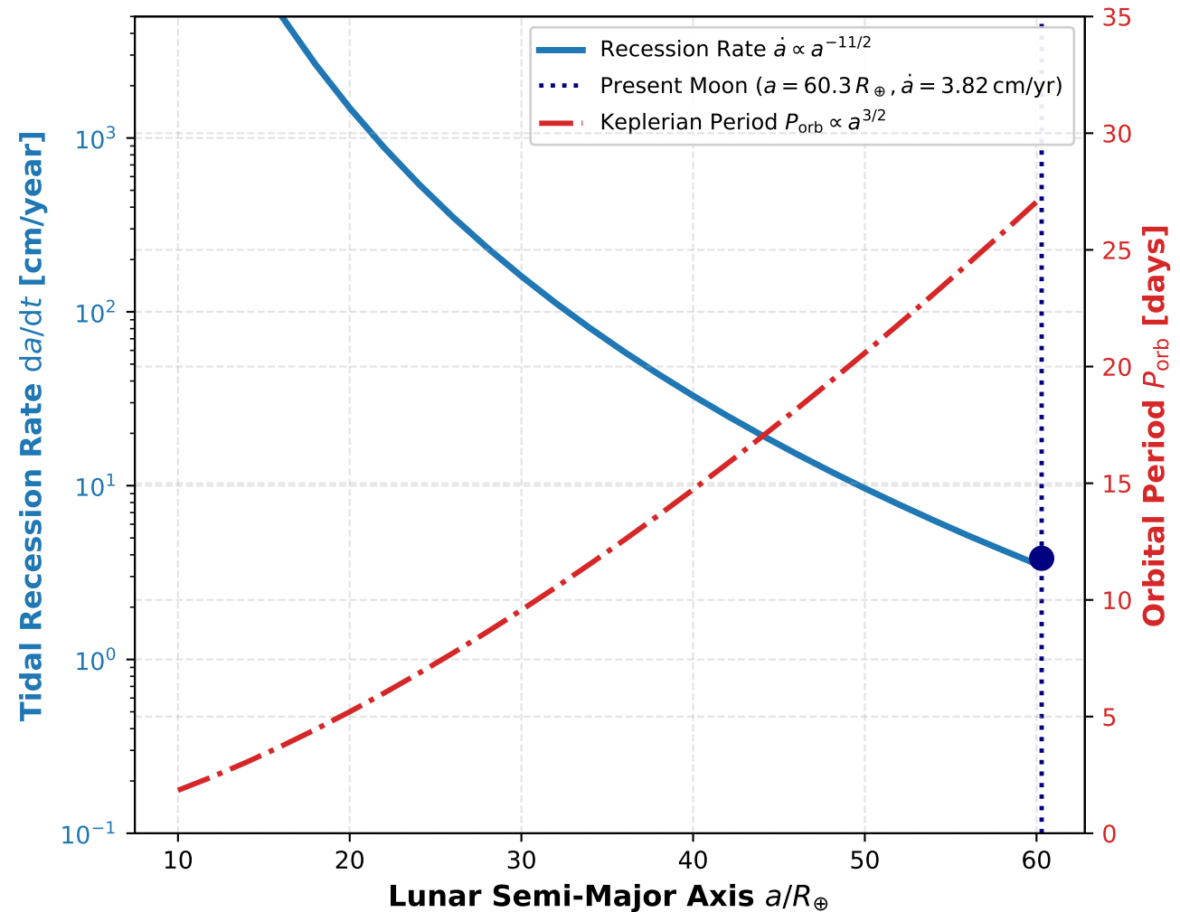
(b) Earth-Moon Recession Dynamics & Keplerian Period
