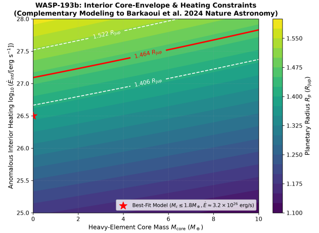
Figure 6: WASP-193b Core-Envelope Constraints. 2D parameter space of heavy-element core mass M_c versus anomalous interior heating \dot{E}_{\text{int}} using the Saumon-Chabrier EOS and Guillot atmosphere. Matching R_p = 1.464 \pm 0.058 R_{\text{Jup}} requires M_c \leq 1.8 M_\oplus and \dot{E}_{\text{int}} \approx 3.2 \times 10^{26} erg/s.
