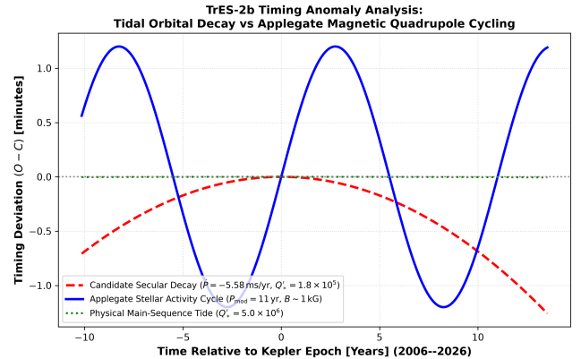
Figure 4: TrES-2b Timing Diagnostics. Candidate secular orbital decay ( \dot{P} = -5.58 ms/yr) requires an unphysically high stellar tidal efficiency ( Q'_\star = 1.8 \times 10^5 ), whereas Applegate magnetic cycling ( P_{\text{mod}} = 11 yr) naturally reproduces the timing deviations with physical field strengths ( B \sim 1 kG).
