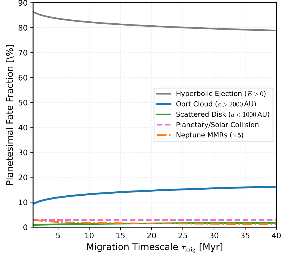
(b) Fate Branching Fractions vs \tau_{\text{mig}}
