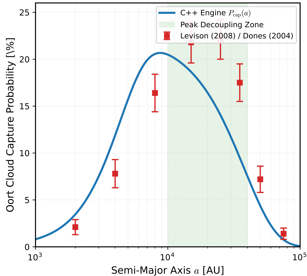
(a) Oort Cloud Capture Efficiency vs a
