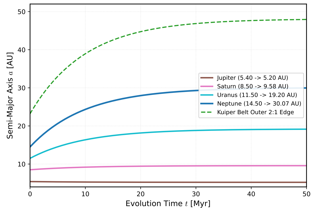
(c) Giant Planet Radial Migration Trajectories
