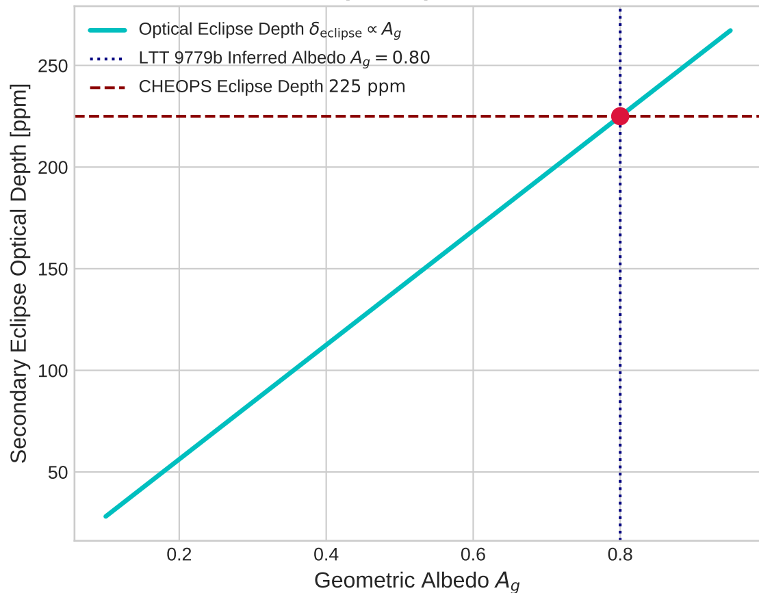
Model Choice: Eclipse Depth vs Geometric Albedo
