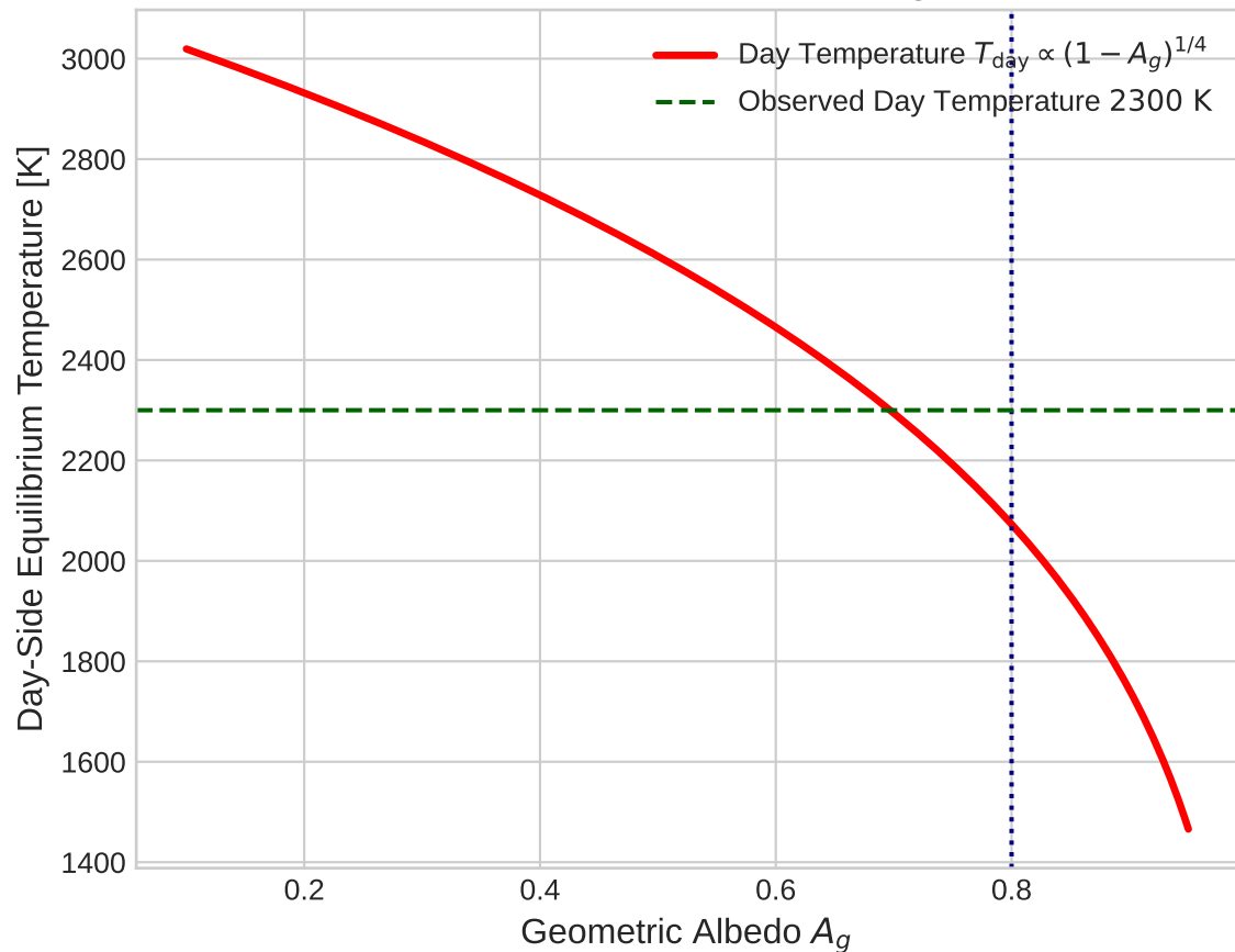
Model Choice: Reflective Cooling Effect
