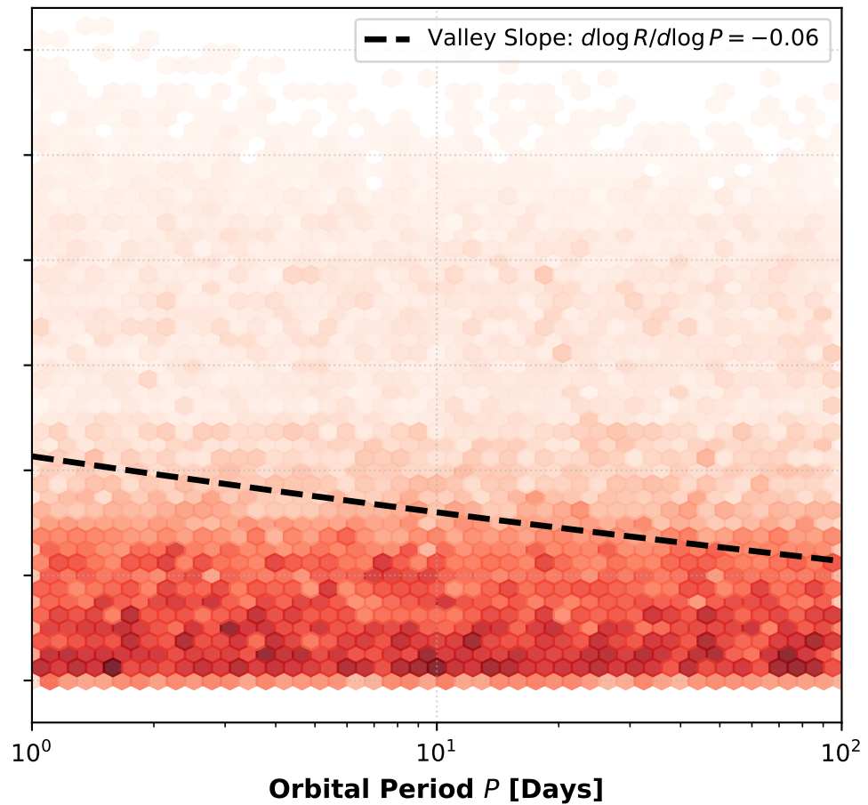
Core-Powered Mass Loss
