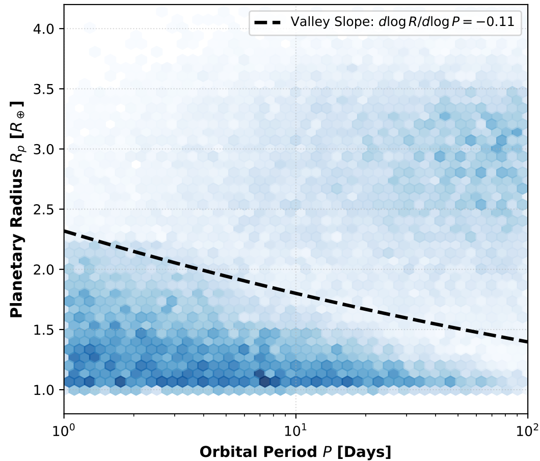
Photoevaporation
