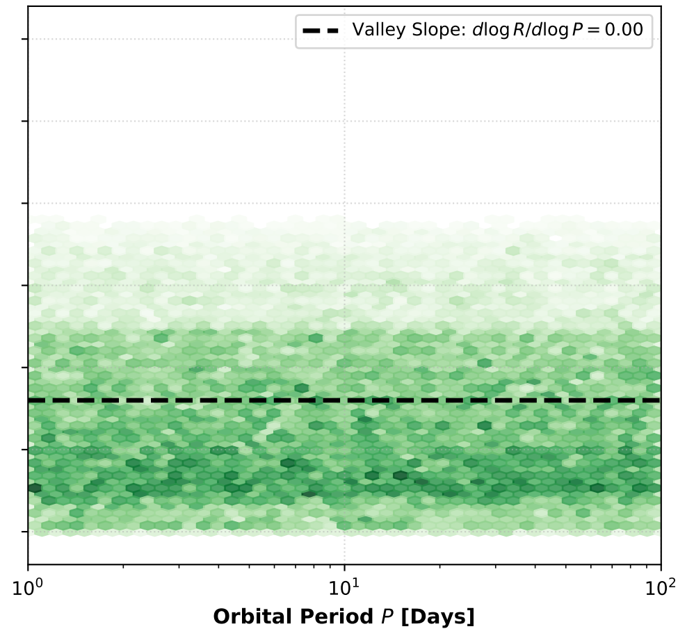
Primordial Water Worlds
