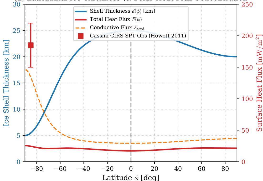
(a) Latitudinal Ice Thickness \& Polar Heat Flux Concentration
