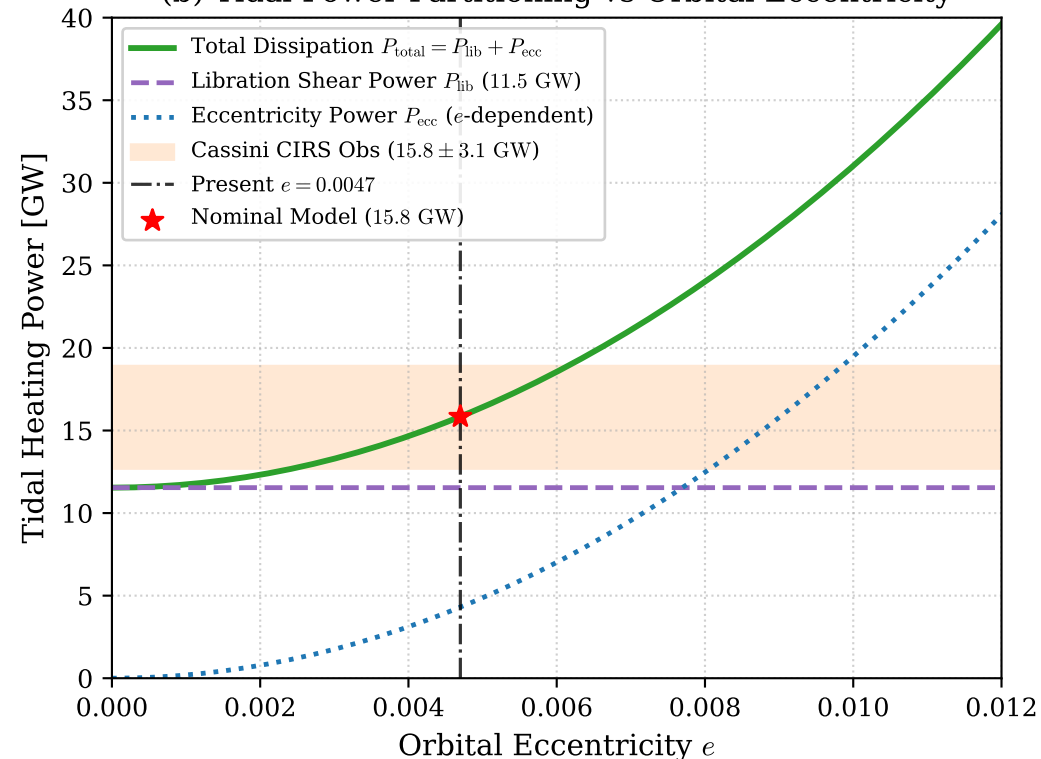
(b) Tidal Power Partitioning vs Orbital Eccentricity
