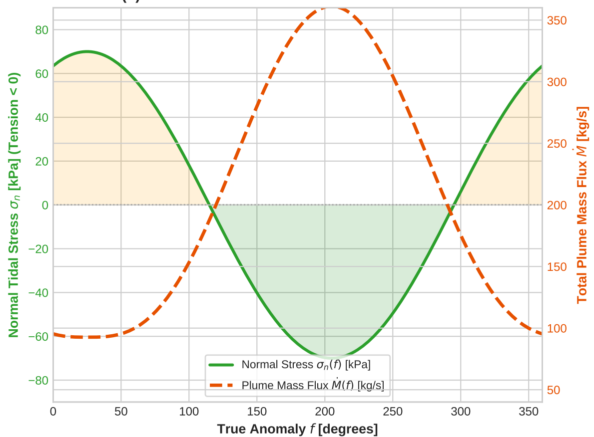
(b) Fracture Normal Stress & Modulated Mass Flux
