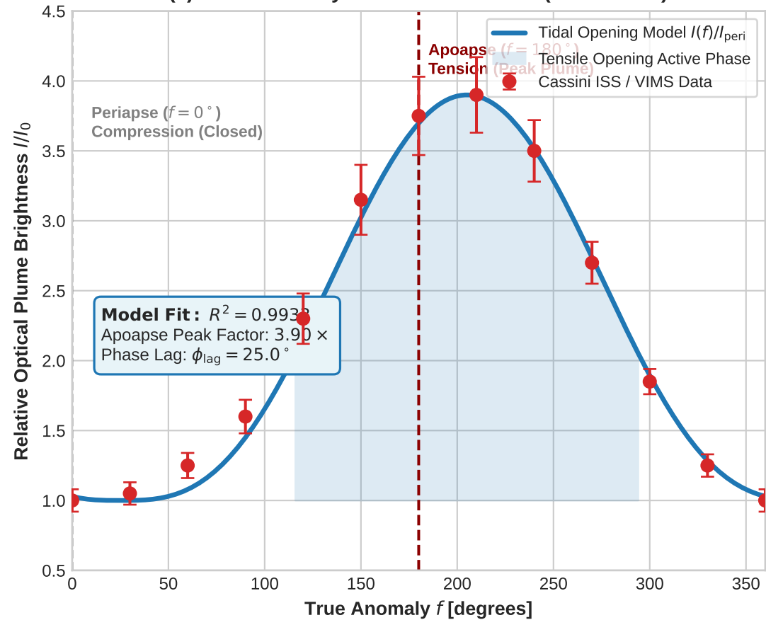
(a) Plume Activity vs. Orbital Position ( R^2 = 0.993 )
