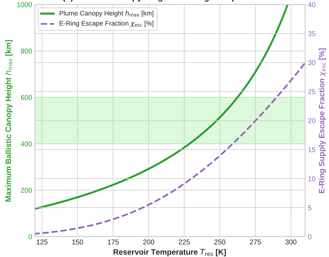
(b) Ballistic Canopy Height & E-Ring Escape Fraction
