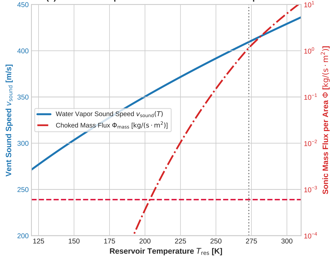
(a) Vent Sound Speed & Choked Mass Flux vs. Temperature
