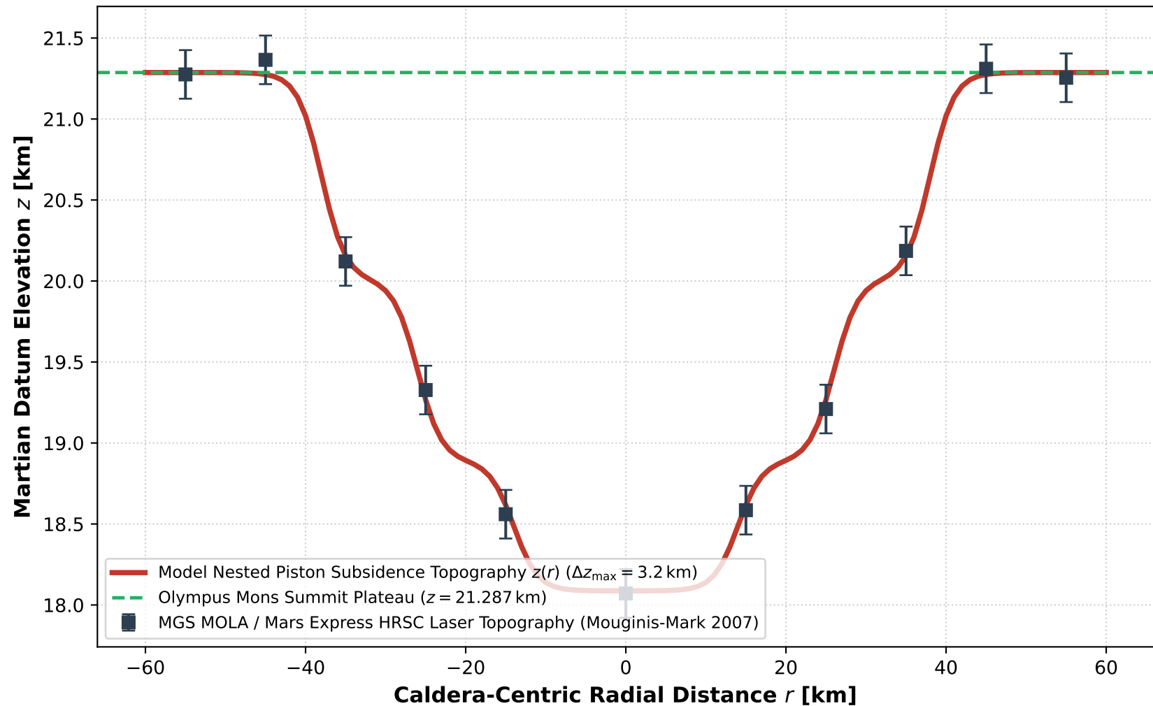
Mars: Olympus Mons Summit Caldera Nested Multi-Ring Subsidence Profile
