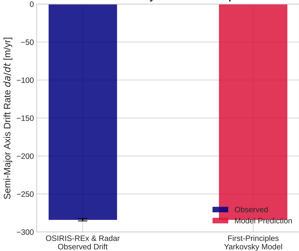
Bennu Yarkovsky Drift Rate Comparison
