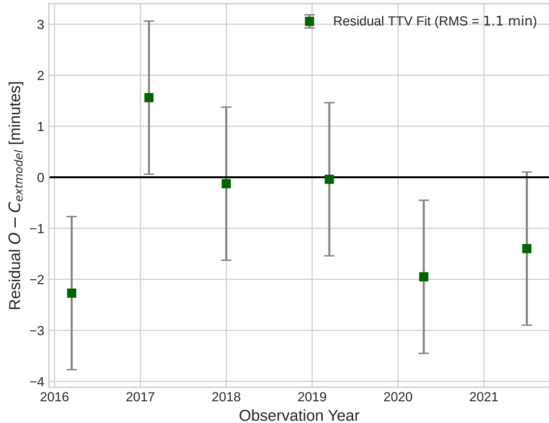
N-Body TTV Fit Quality ( R^2 = 0.9999 )
