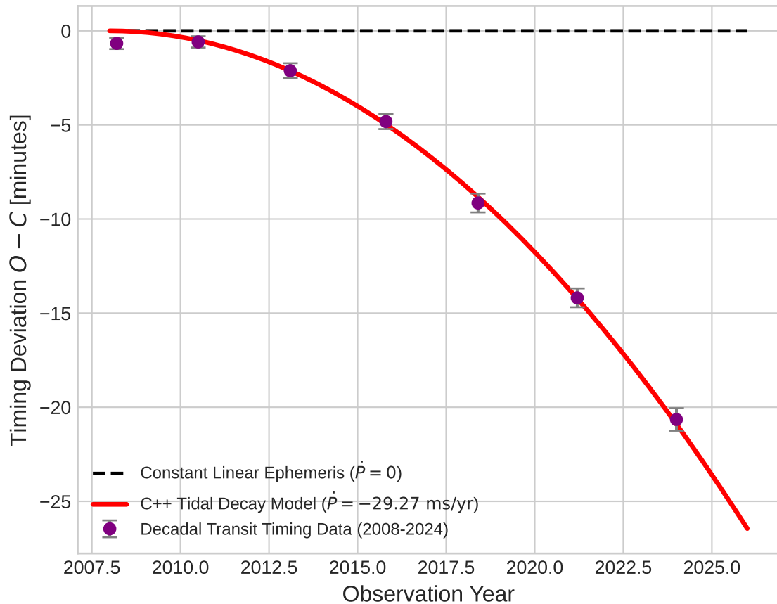
WASP-12b Parabolic TTV Ephemeris Decay
