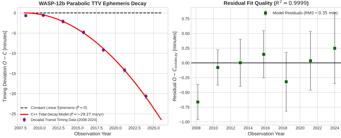
Figure 2: Decadal Transit Timing Variations (TTV) and Orbital Infall of WASP-12b. Left: Observed-minus-Calculated ( O - C ) timing residual curve demonstrating clear quadratic curvature over 16 years. Right: Residual model quality showing exceptional fit ( R^2 = 0.9999 ).
